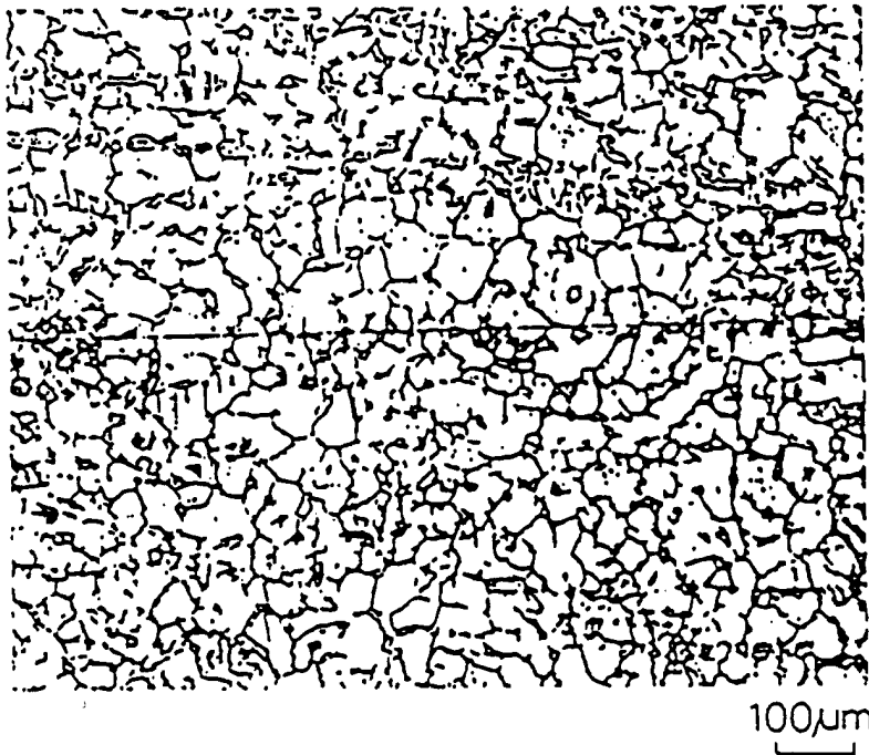
Fig. 5 ( HEAT TREATING PROCESS C )
