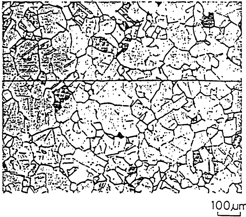
Fig. 4 ( HEAT TREATING PROCESS B )
