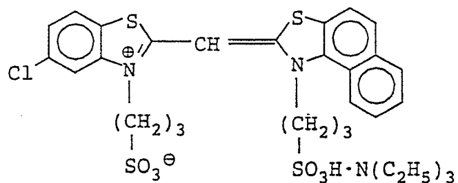
Sensitizing Dye B for blue-sensitive emulsion layer
