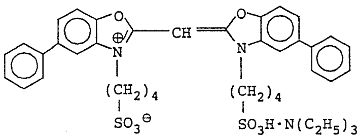
Sensitizing Dye D for green-sensitive emulsion layer
