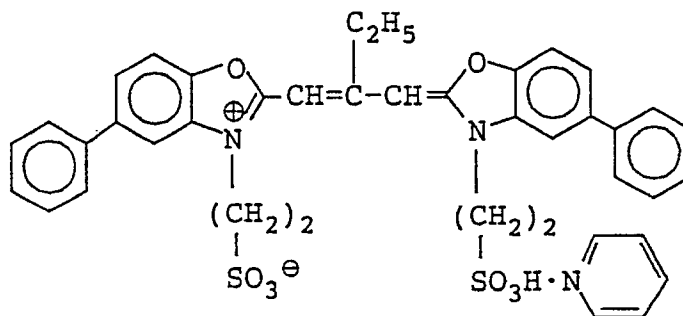
Sensitizing Dye A for green-sensitive emulsion layer
