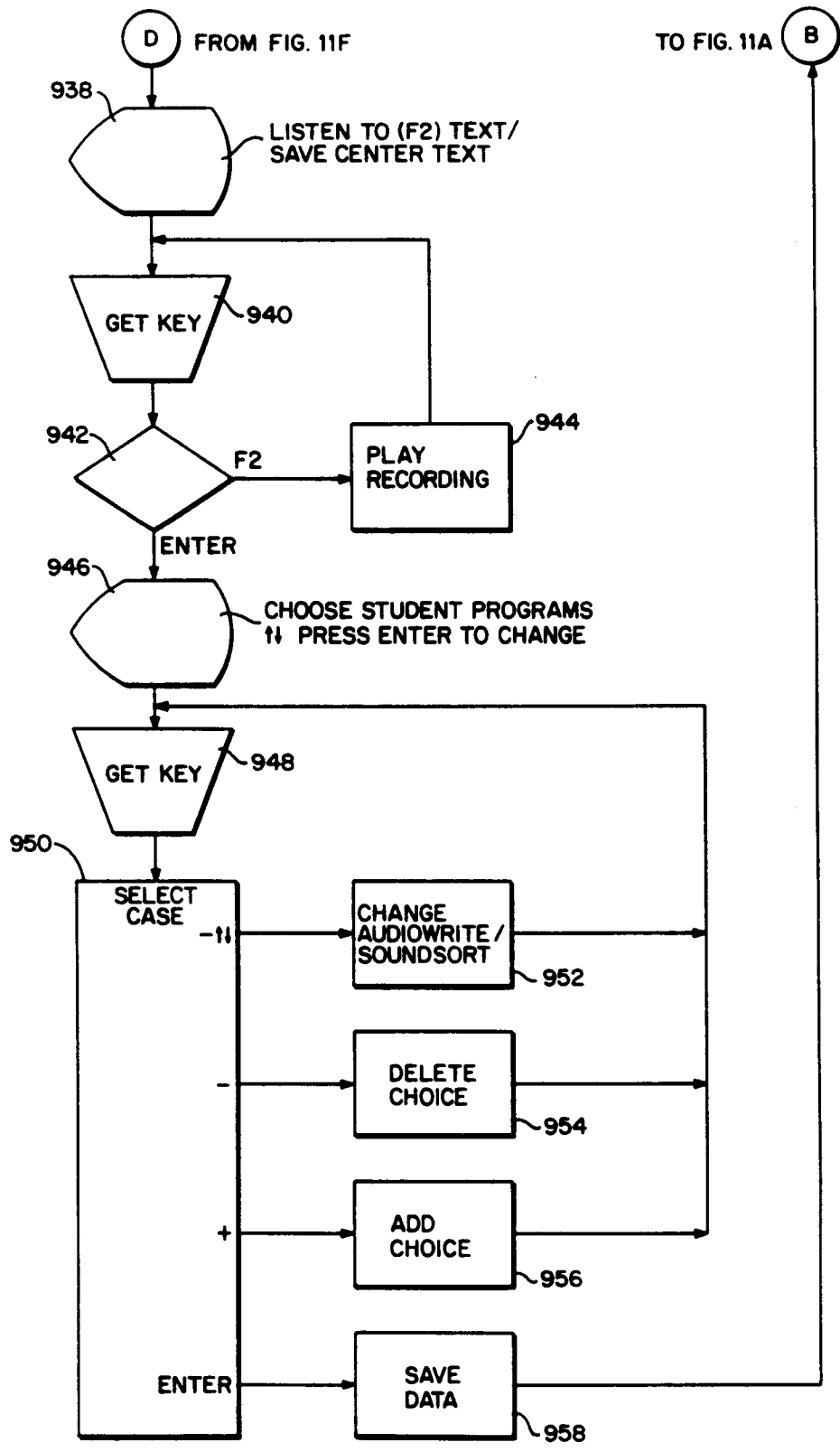
FIG.11G "STUDIO" ROUTINE
