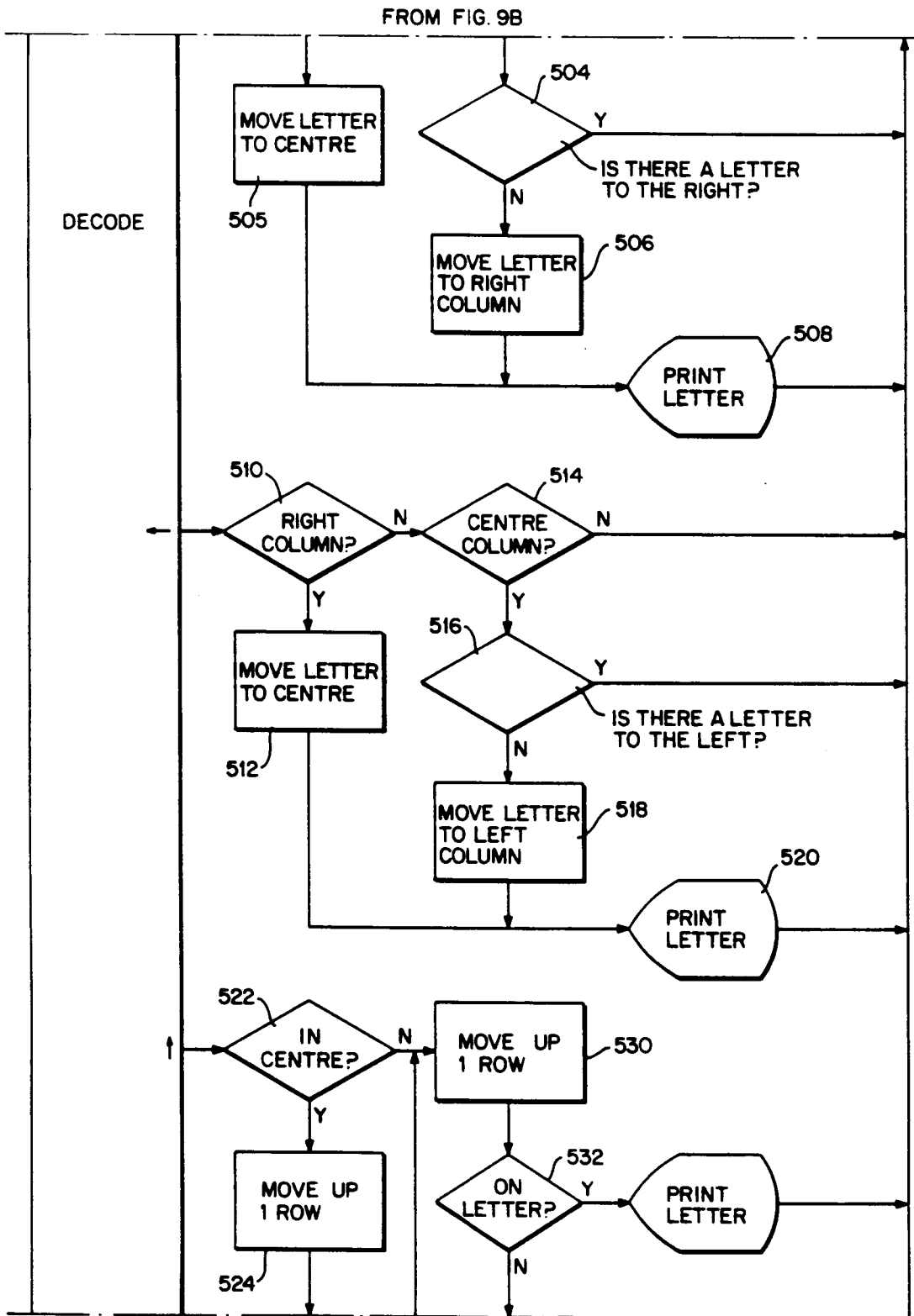
FIG. 9C "SOUND SORT" ROUTINE
