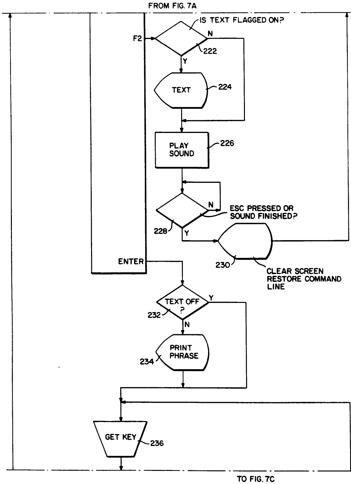
FIG. 7B "AUDIO LAB" ROUTINE
