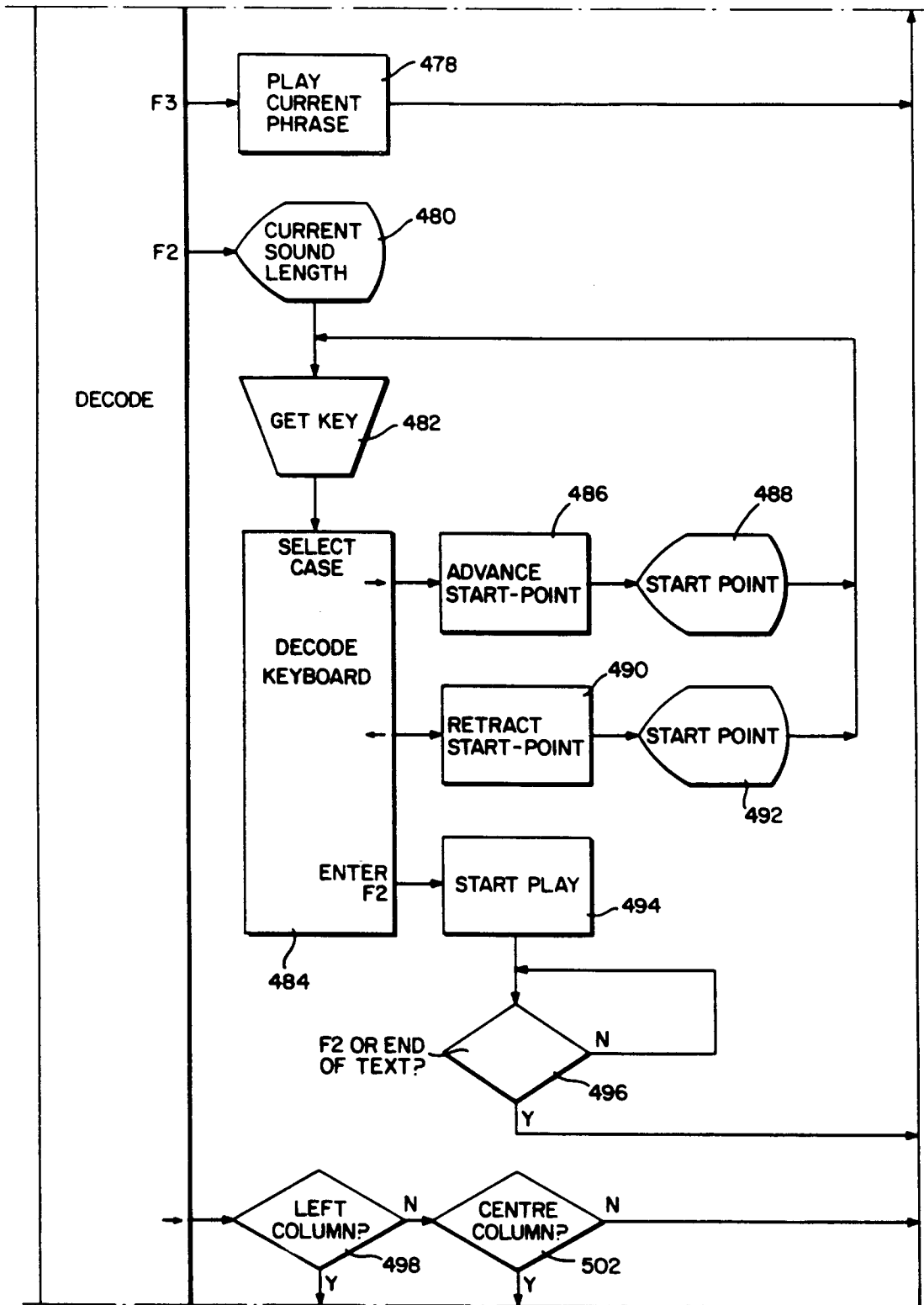
FIG. 9B "SOUND SORT" ROUTINE
