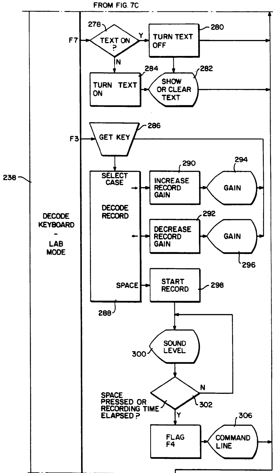
FIG. 7D "AUDIO LAB" ROUTINE
