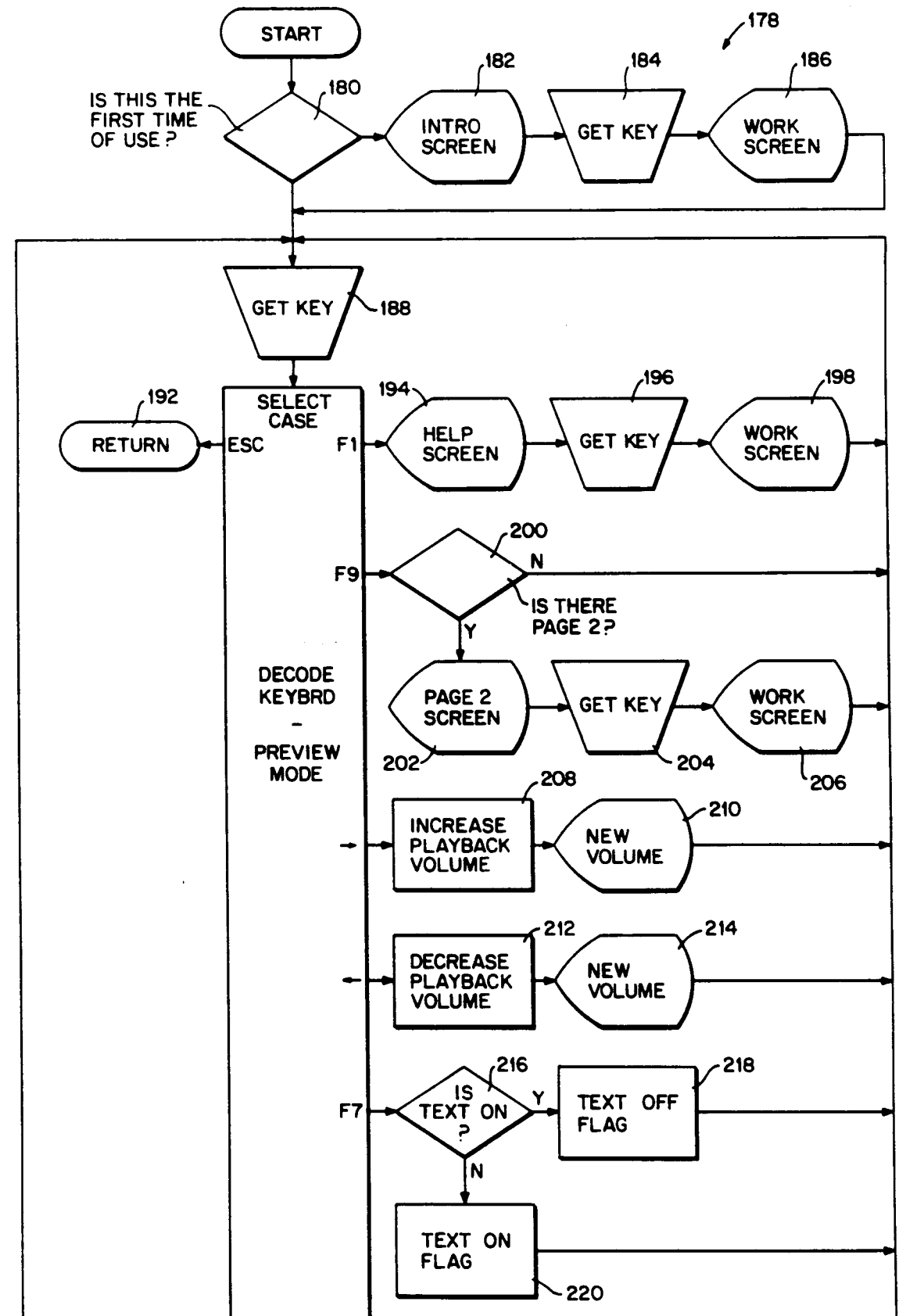
FIG. 7A "AUDIO LAB" ROUTINE
