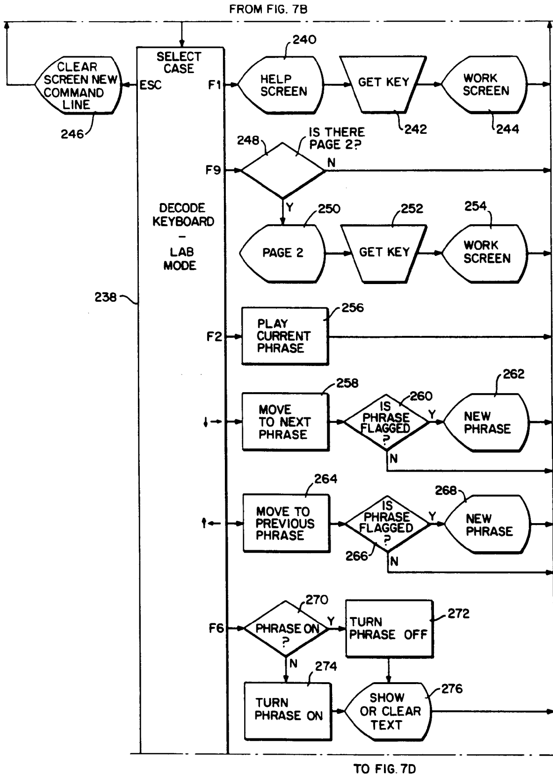
FIG. 7C "AUDIO LAB" ROUTINE
