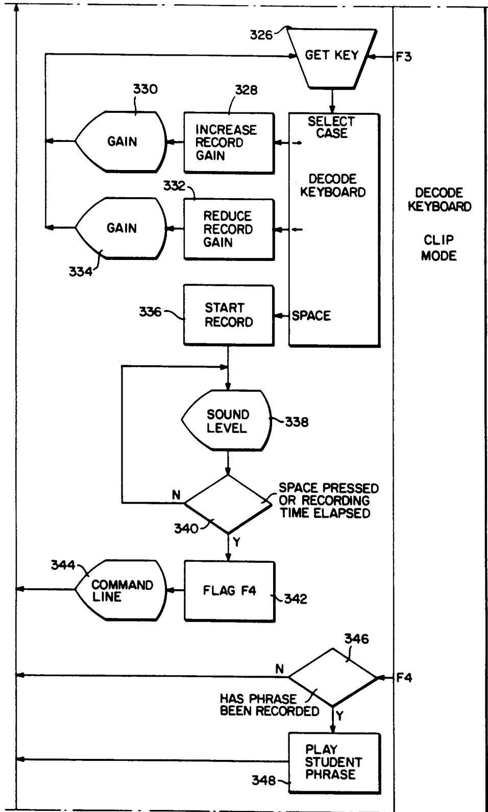
FIG. 7F "AUDIO LAB" ROUTINE
