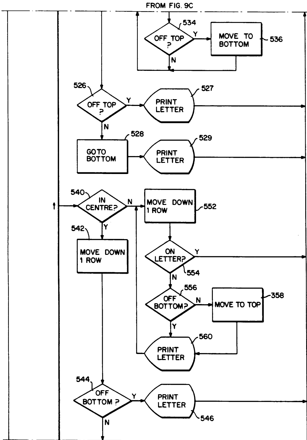
FIG. 9D "SOUND SORT" ROUTINE
