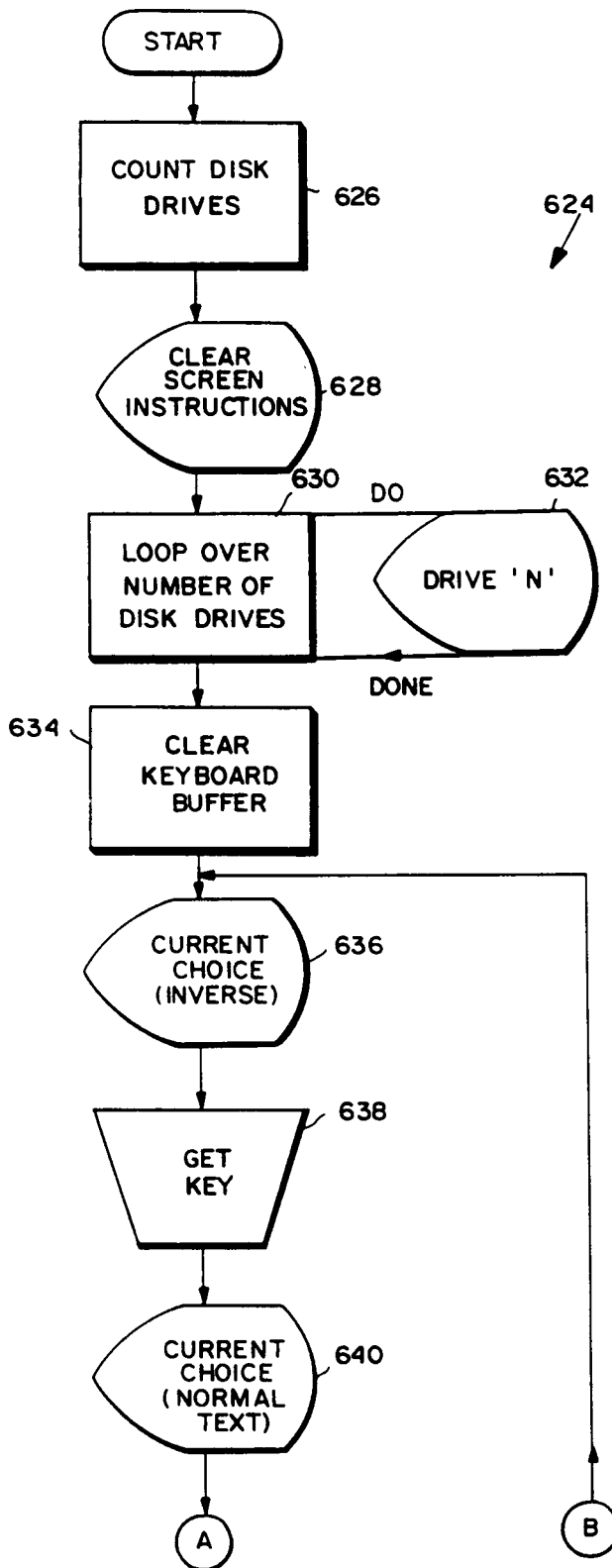
FIG. 13A "CHOOSE DRIVE" ROUTINE
