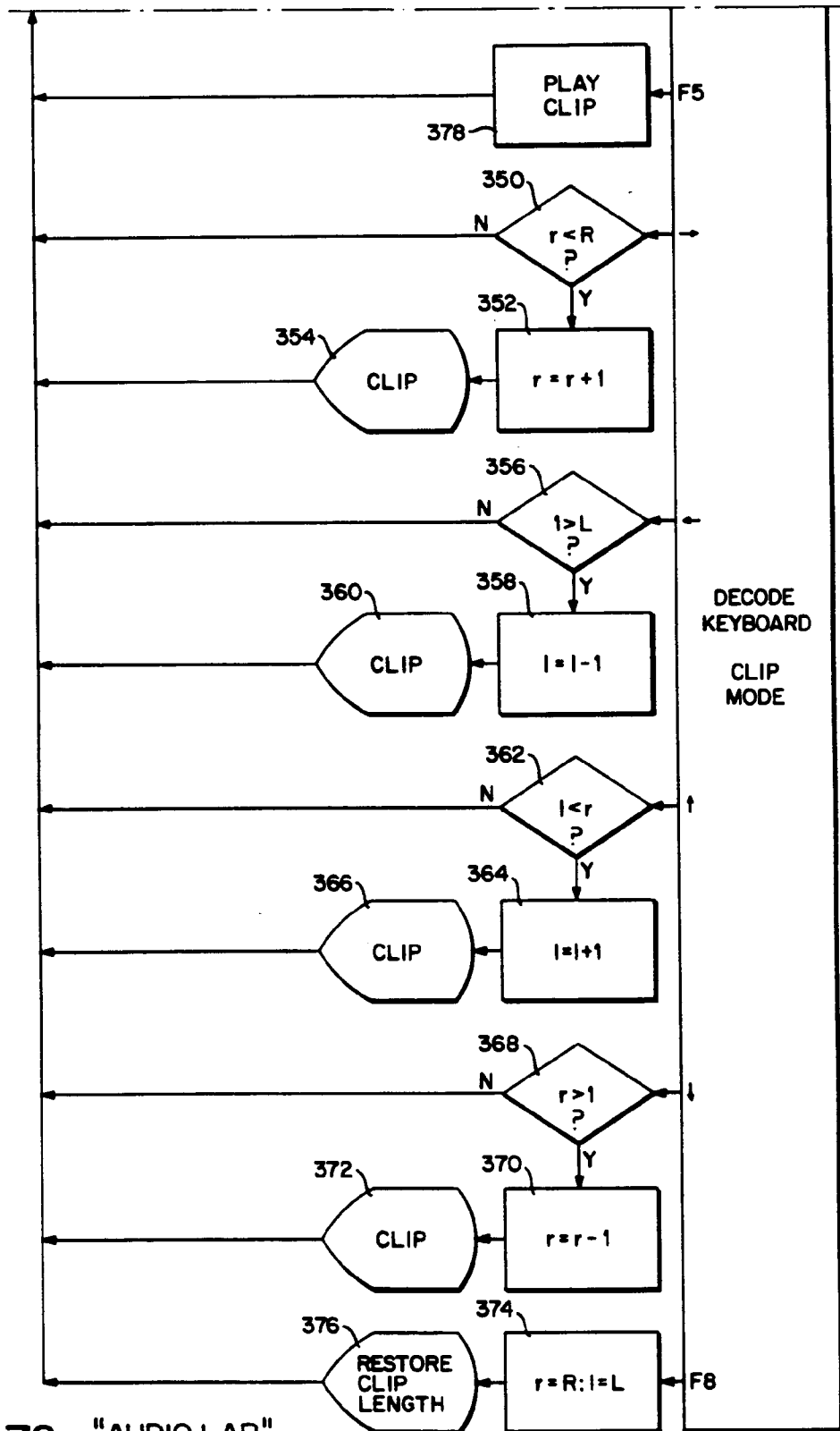
FIG. 7G "AUDIO LAB" ROUTINE
