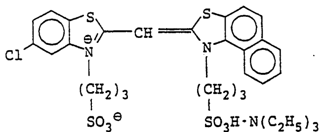
Sensitizing dye B for blue-sensitive emulsion layer
