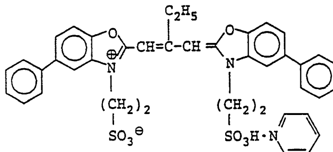
Sensitizing dye C for green-sensitive emulsion layer
