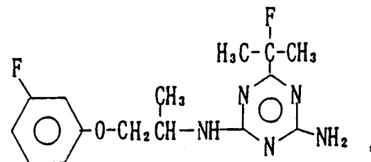
2-amino-4-( \alpha -fluoro, \alpha -methylethyl)-6-[2-(3'fluorophenoxy)-1-methylethylamino]-s-triazine
