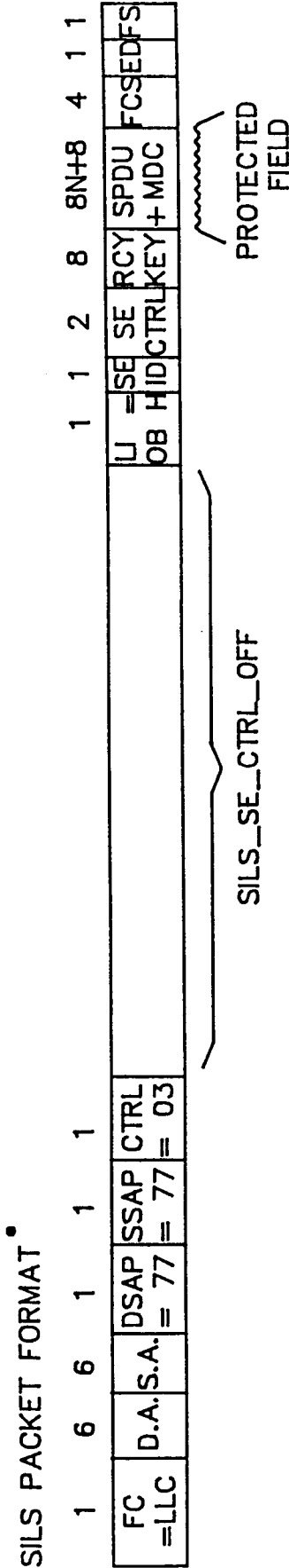
FIG. 11 SILS ENCRYPTION
