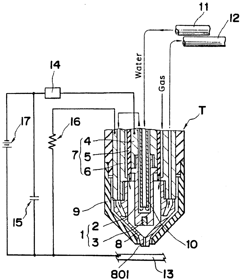
Fig. 7 PRIOR ART
