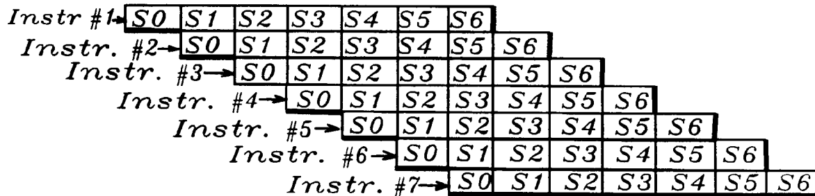
FIG 7 PIPELINE
