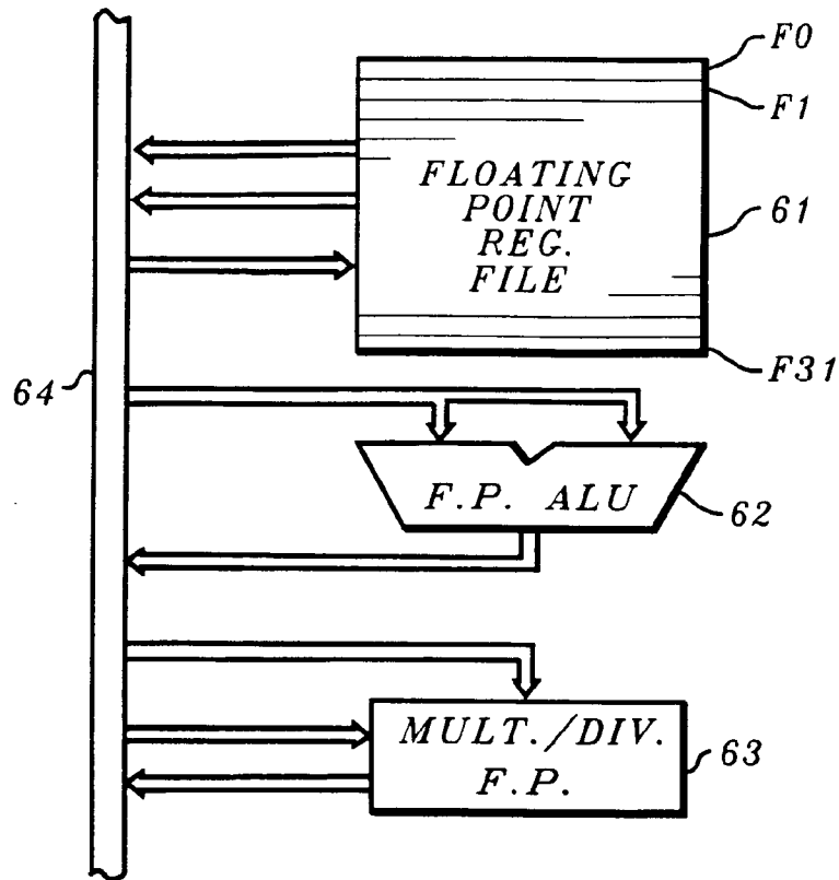
FIG 6 F-BOX
