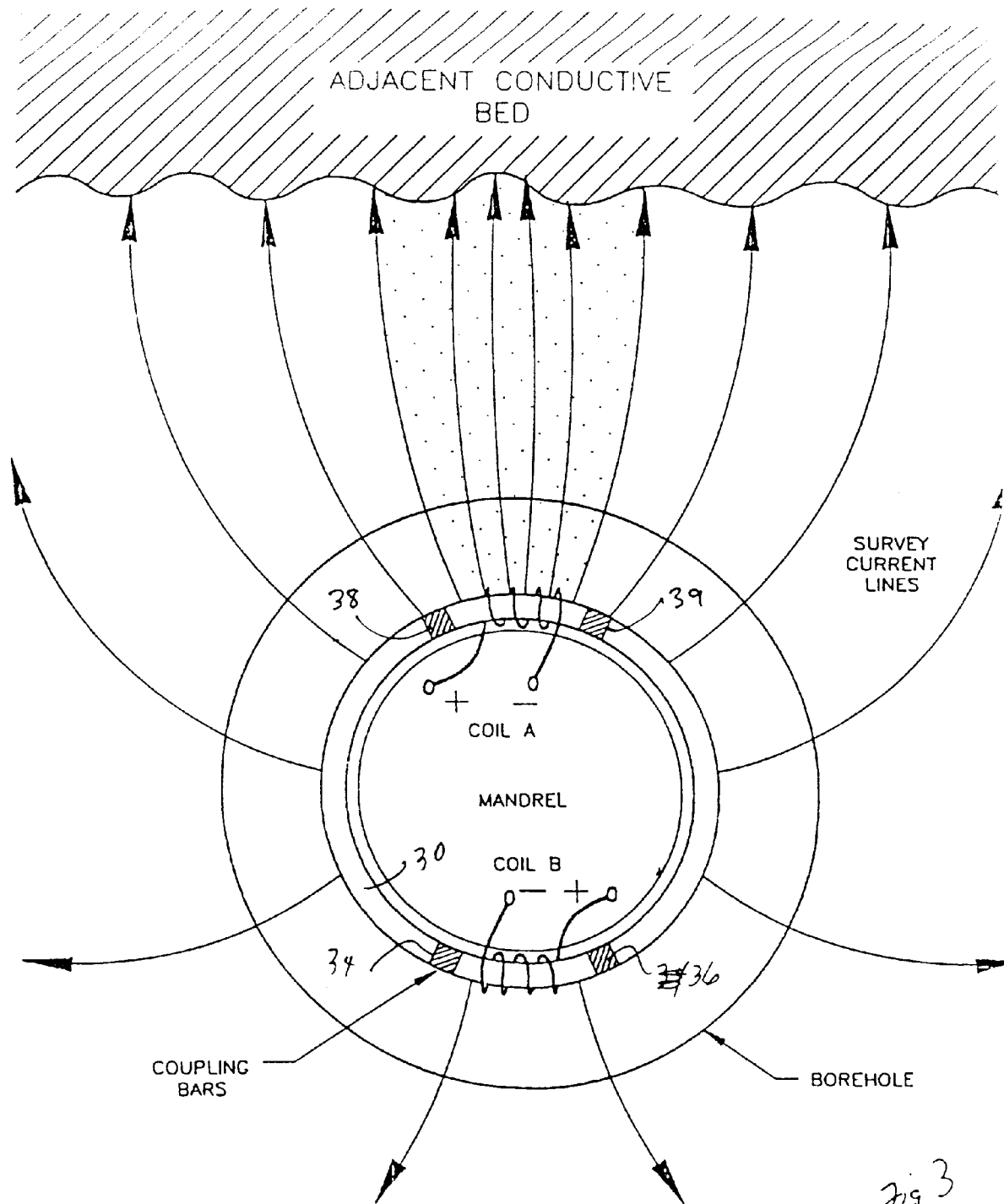
SECTIONAL VIEW OF AZIMUTHAL FOCUSSED MWD RESISTIVITY
