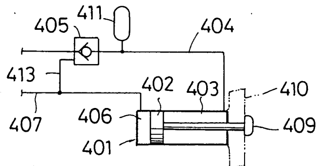
Fig. 21 PRIOR ART
