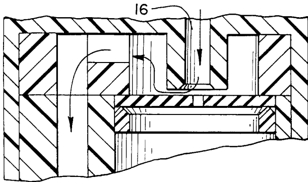
FIG. 1 PRIOR ART
