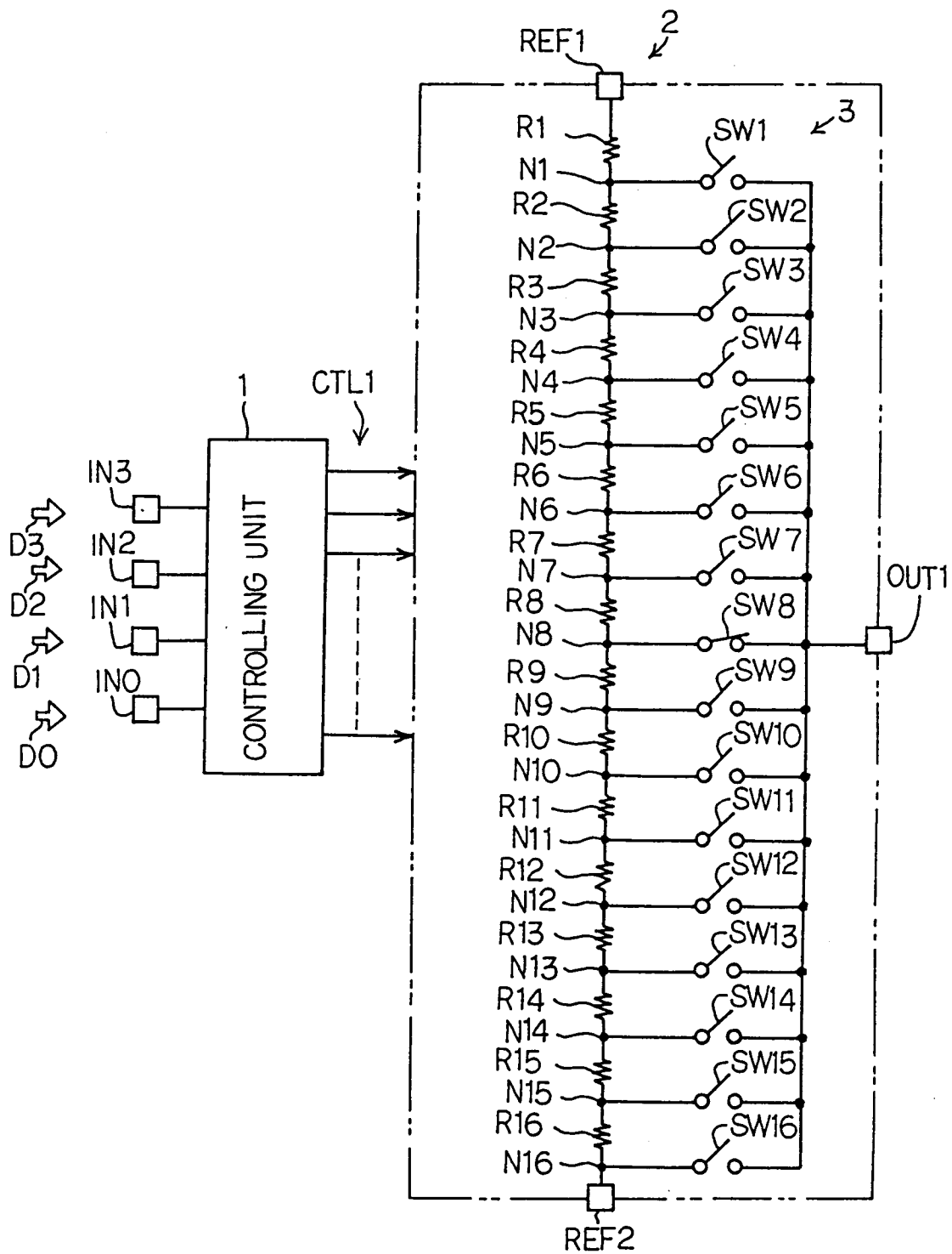
Fig. 1 PRIOR ART
