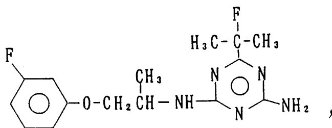
2-amino-4-(α-fluoro,α-methylethyl)-6-[2-(3'-fluorophenoxy)-1-methylethylamino]-s-triazine
