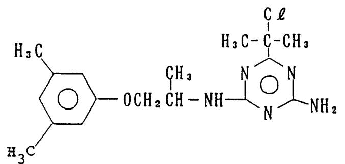
2-amino-4-(α-fluoro,α-methylethyl)-6-[2-(3',5'-dimethylphenoxy)-1-methylethylamino]-s-triazine
