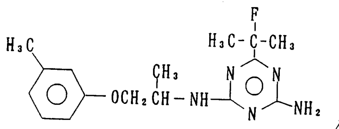
2-amino-4-(α-fluoro,α-methylethyl)-6-[2-(3'-fluorophenoxy)-1-methylethylamino]-s-triazine
