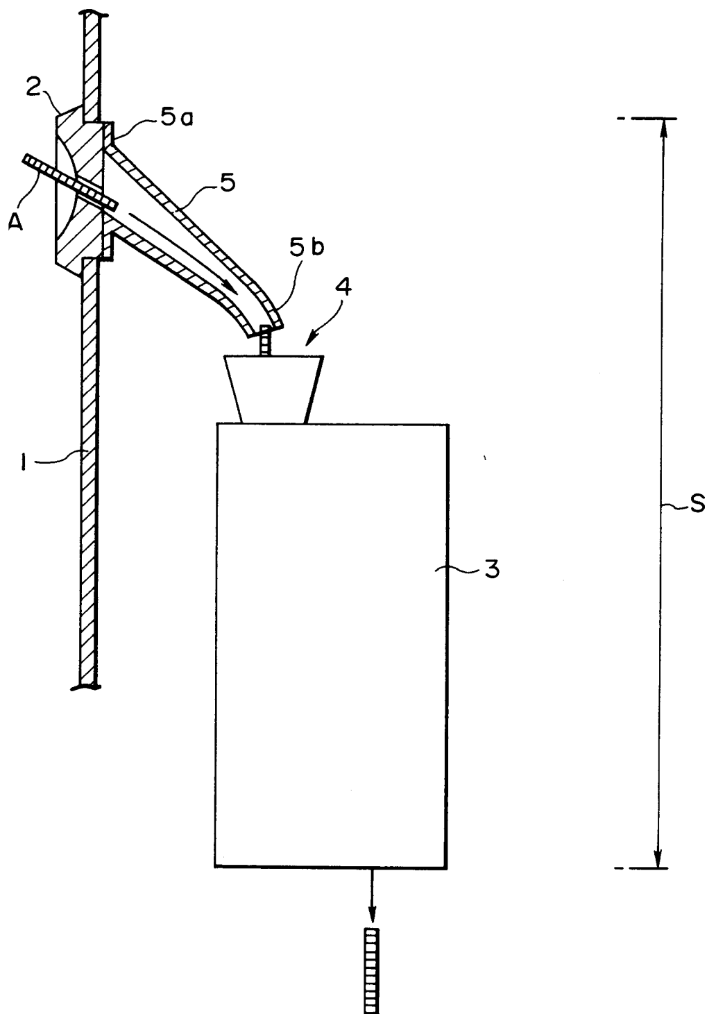
FIG. 13 (PRIOR ART)
