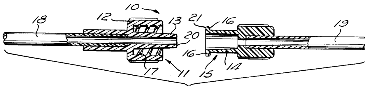
Fig. 1 (PRIOR ART)
