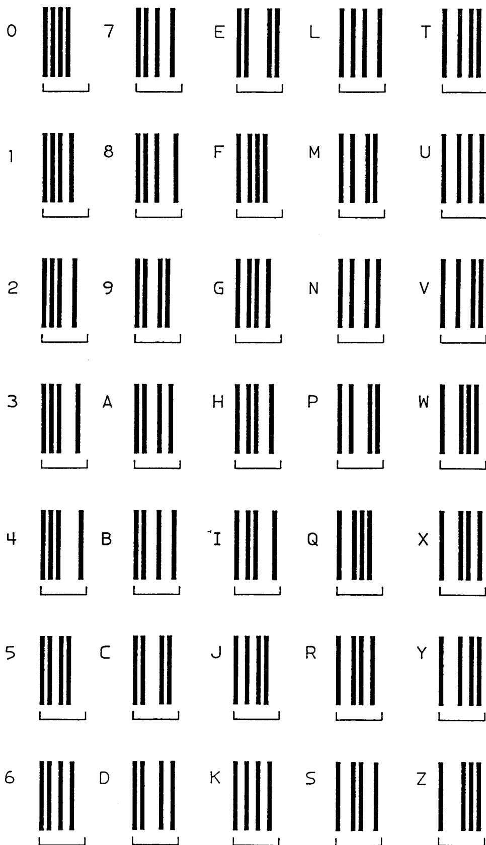
FIG. 1 CHARACTER FONT BAR PATTERNS CODE BC412
