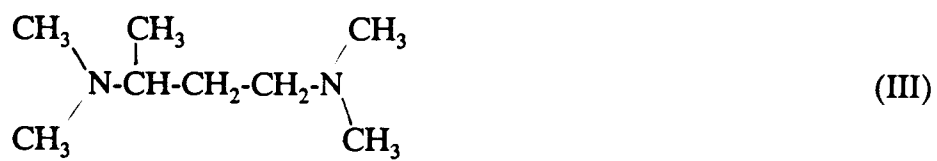
N,N,N',N'-tetramethyl-1,3-butane diamine
