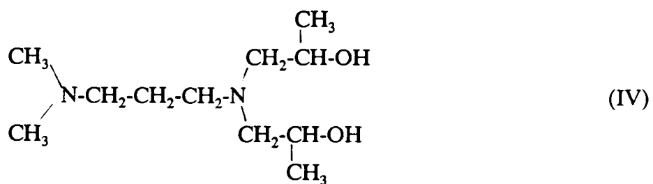
N,N-dimethyl-N',N'-di(2-hydroxypropyl)-1,3-propane diamine
