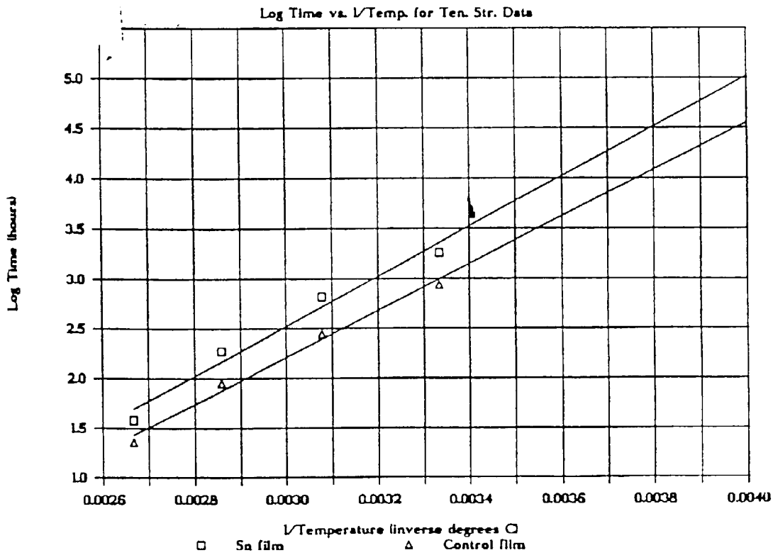
THERMAL DURABILITY
