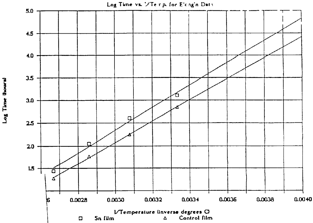
FIGURE 3 THERMAL DURABILITY
