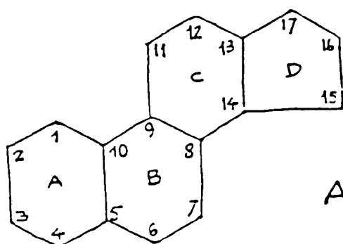
PERHYDROCYCLOPENTANOPHENANTHRENE
