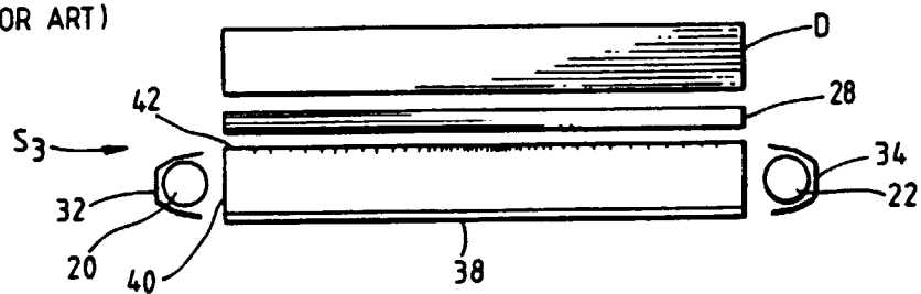
FIG.4 (PRIOR ART)
