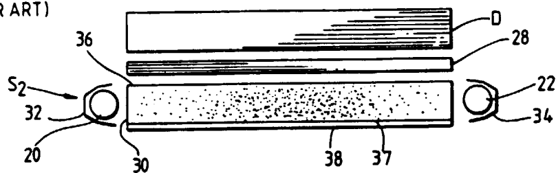
FIG.2 (PRIOR ART)
