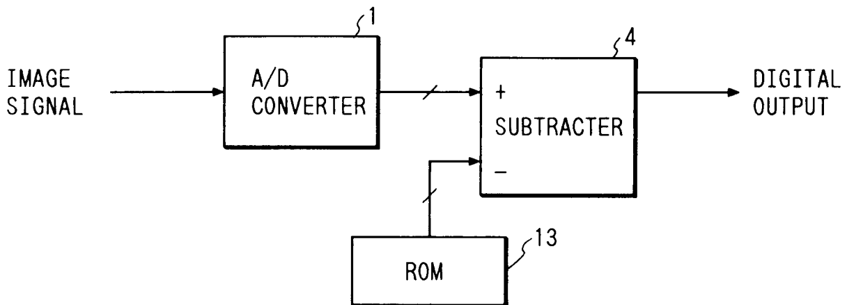
FIG. 2 PRIOR ART
