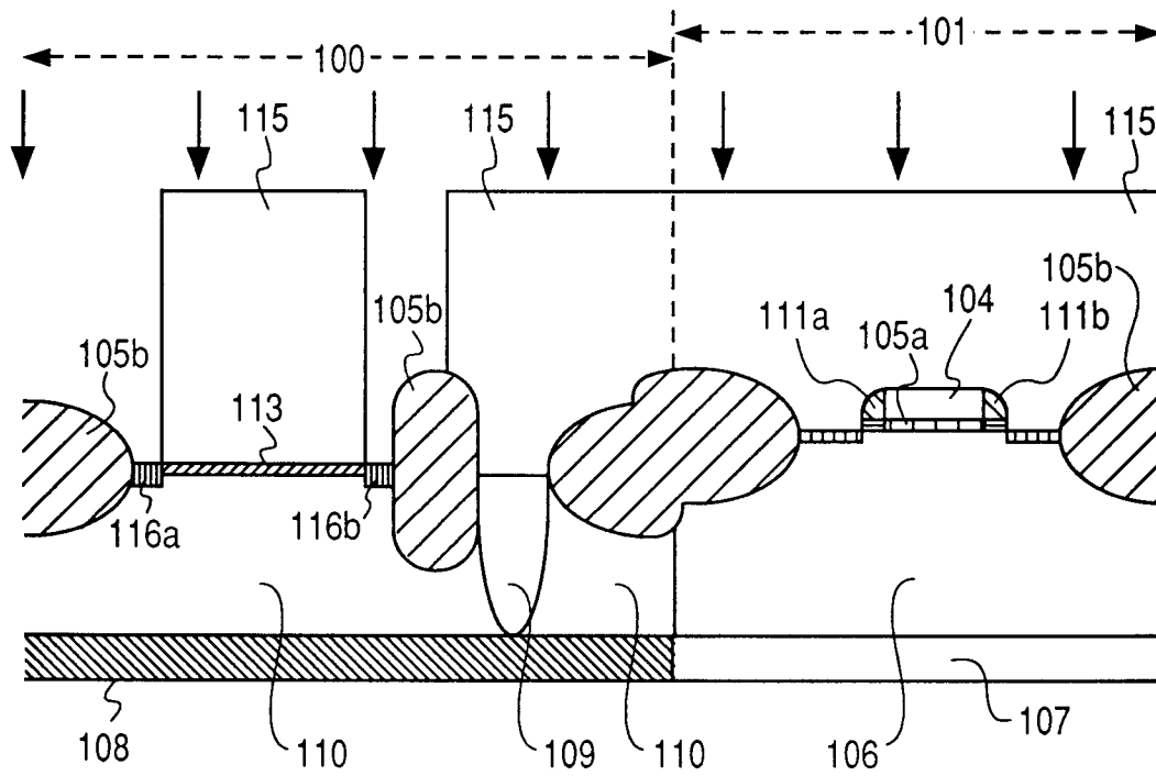
FIG. 1g (PRIOR ART)
