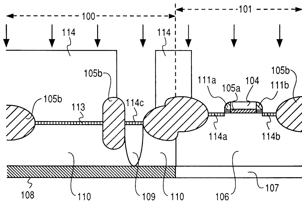
FIG. 1f (PRIOR ART)
