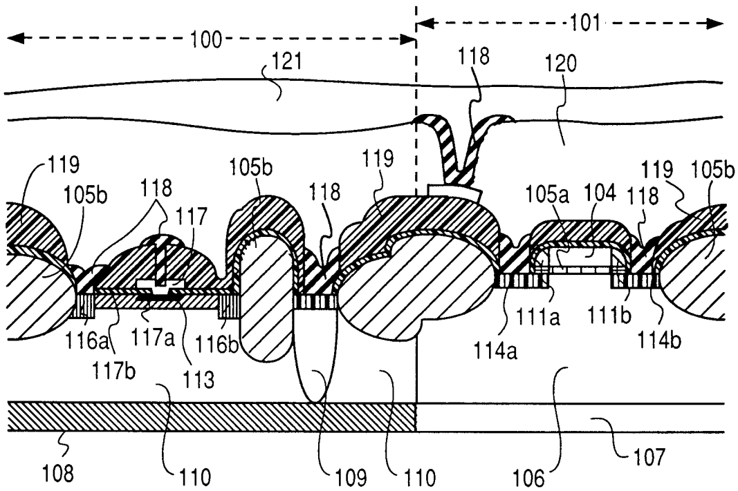
FIG. 1h (PRIOR ART)
