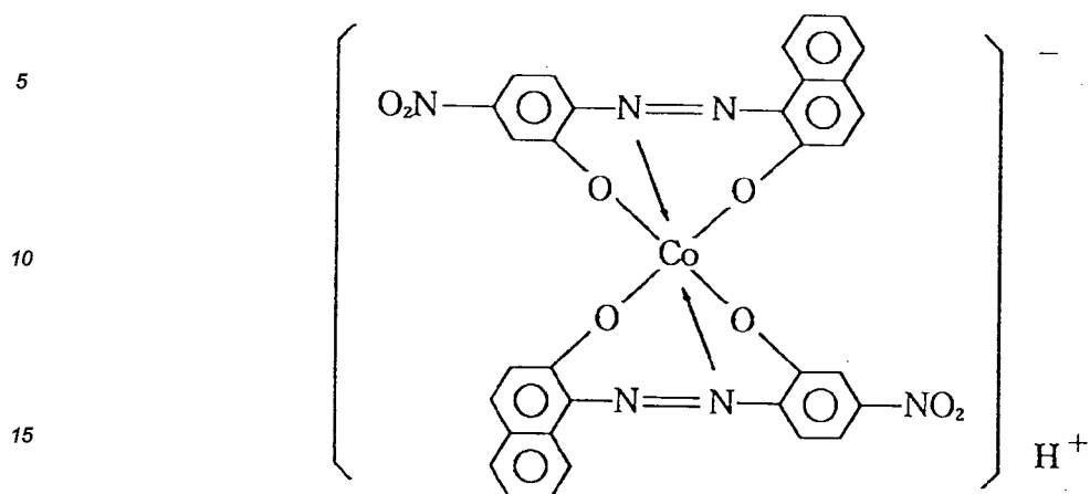
Complex (I)-3
