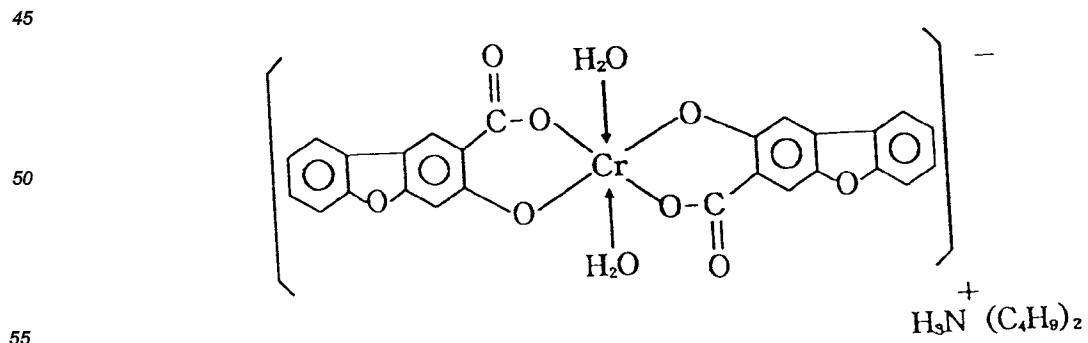
Complex (II)-5
