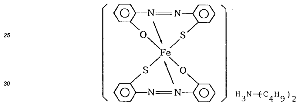
Complex (I)-4
