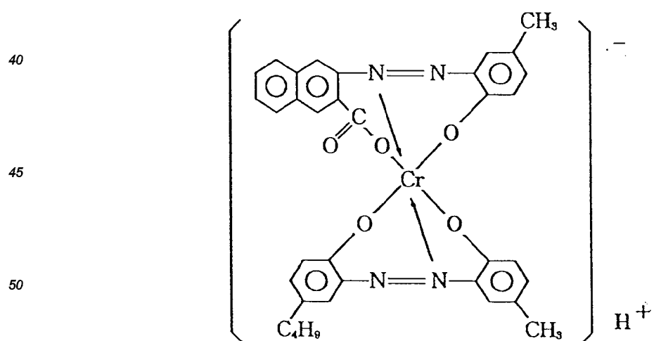
Complex (I)-4
