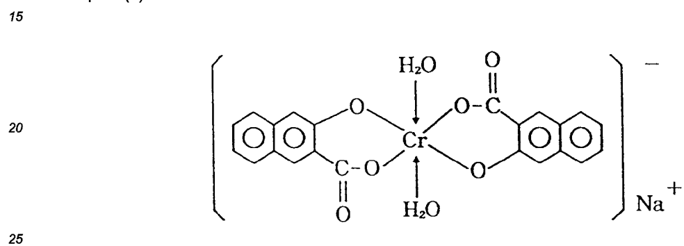
Complex (II)-3
