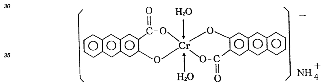
Complex (II)-4
