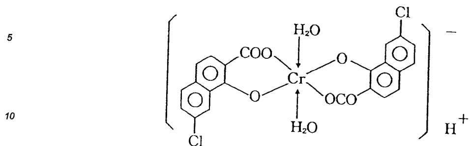
Complex (II)-3
