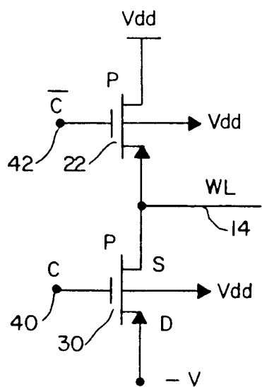
FIG. 2 (PRIOR ART)
