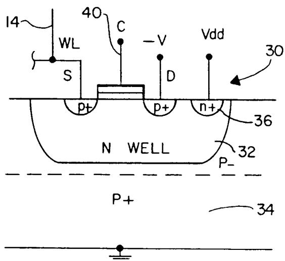
FIG. 3 (PRIOR ART)
