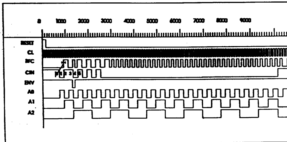
Waveforms with no gap detection or synchronization
