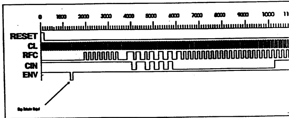
Waveforms with gap detection and synchronization
