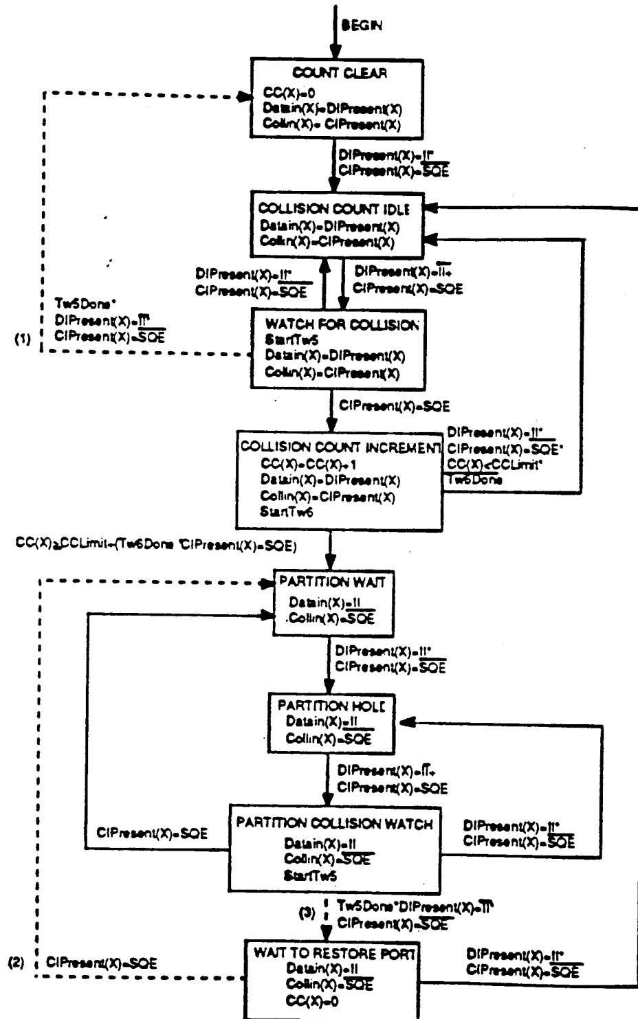
FIG. 29 (PRIOR ART)
