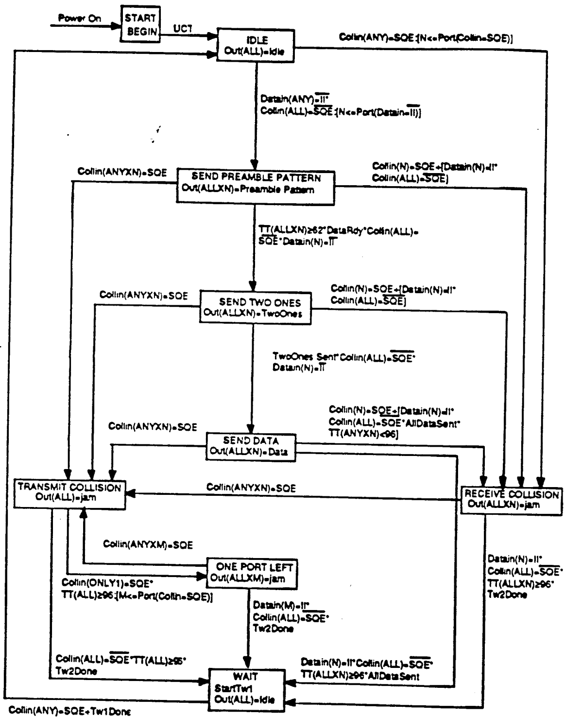
FIG. 10 (PRIOR ART)
