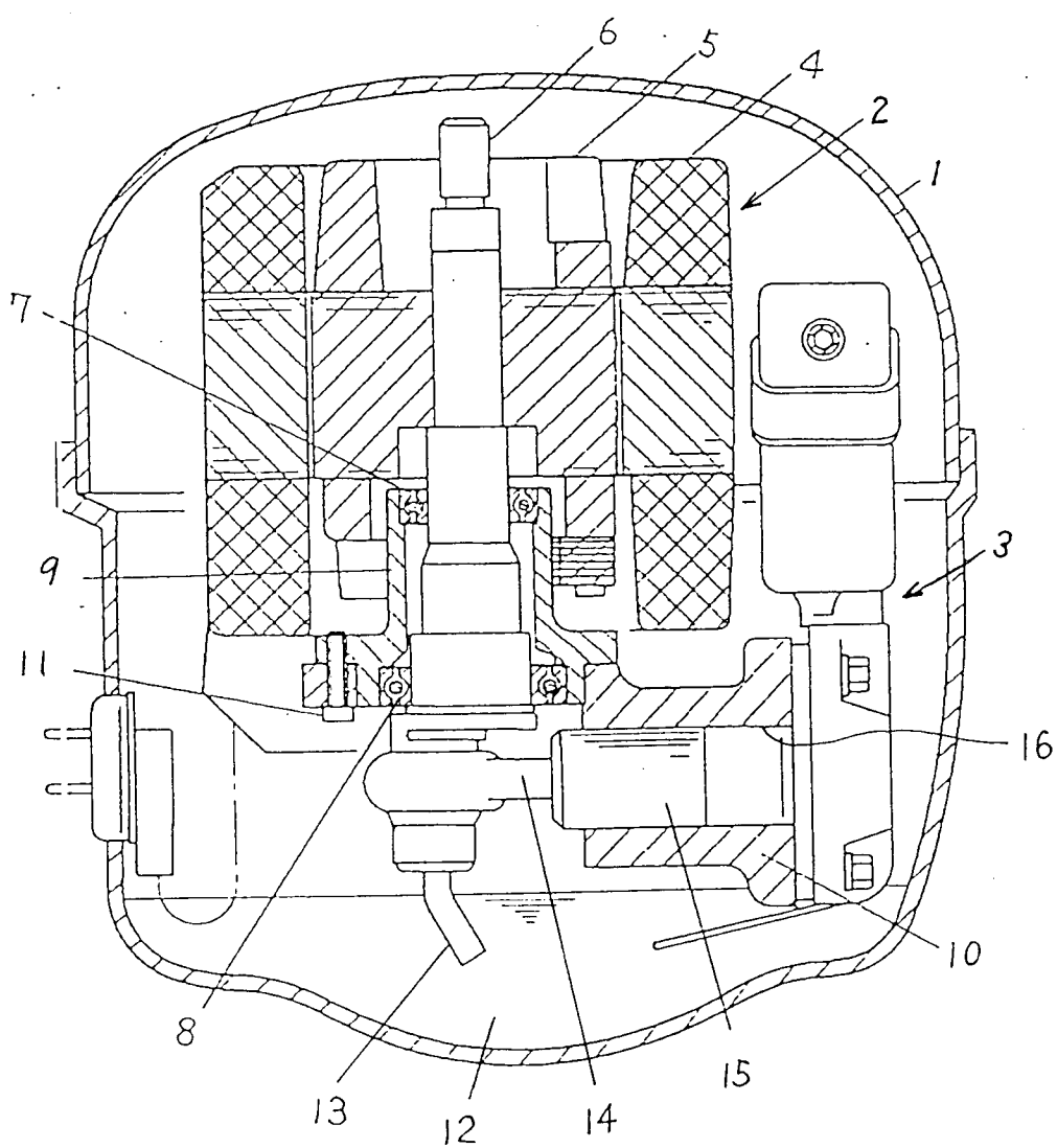
FIG.5 PRIOR ART
