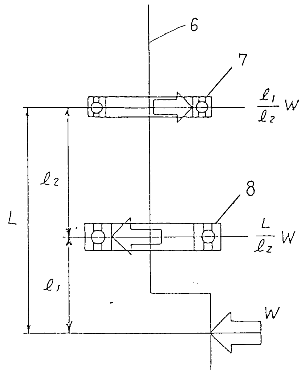
FIG. 6 PRIOR ART
