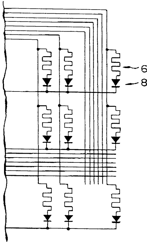
FIG. 49 (PRIOR ART)
