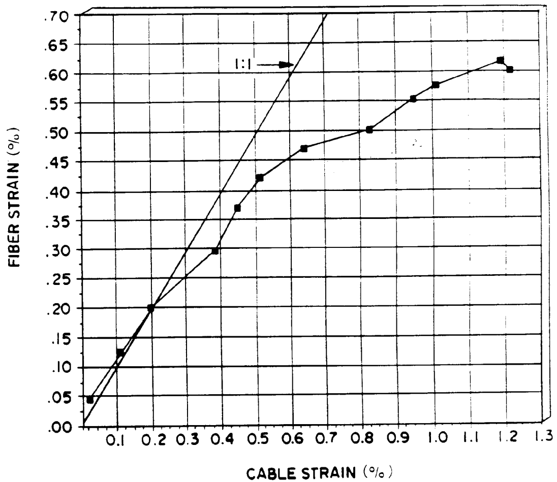
FIBER STRAIN VS. CABLE STRAIN 12 FIBER DESIGN
