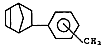
5-Tolyl-bicyclo[2.2.1]hept-2-ene
