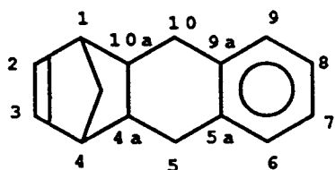
1,4-Methano-1,4,4a,5,10,10a-hexahydroanthracene
