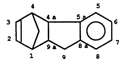
1,4-Methano-1,4,4a,9a-tetrahydrofluorene
