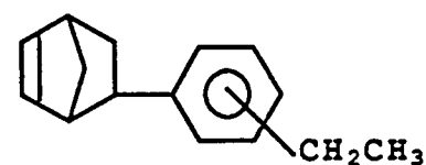
5-(Ethylphenyl)-bicyclo-[2.2.1]hept-2-ene
