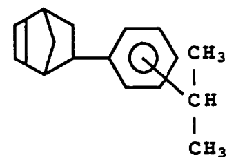
5-(Isopropylphenyl)-bicyclo-[2.2.1]hept-2-ene
