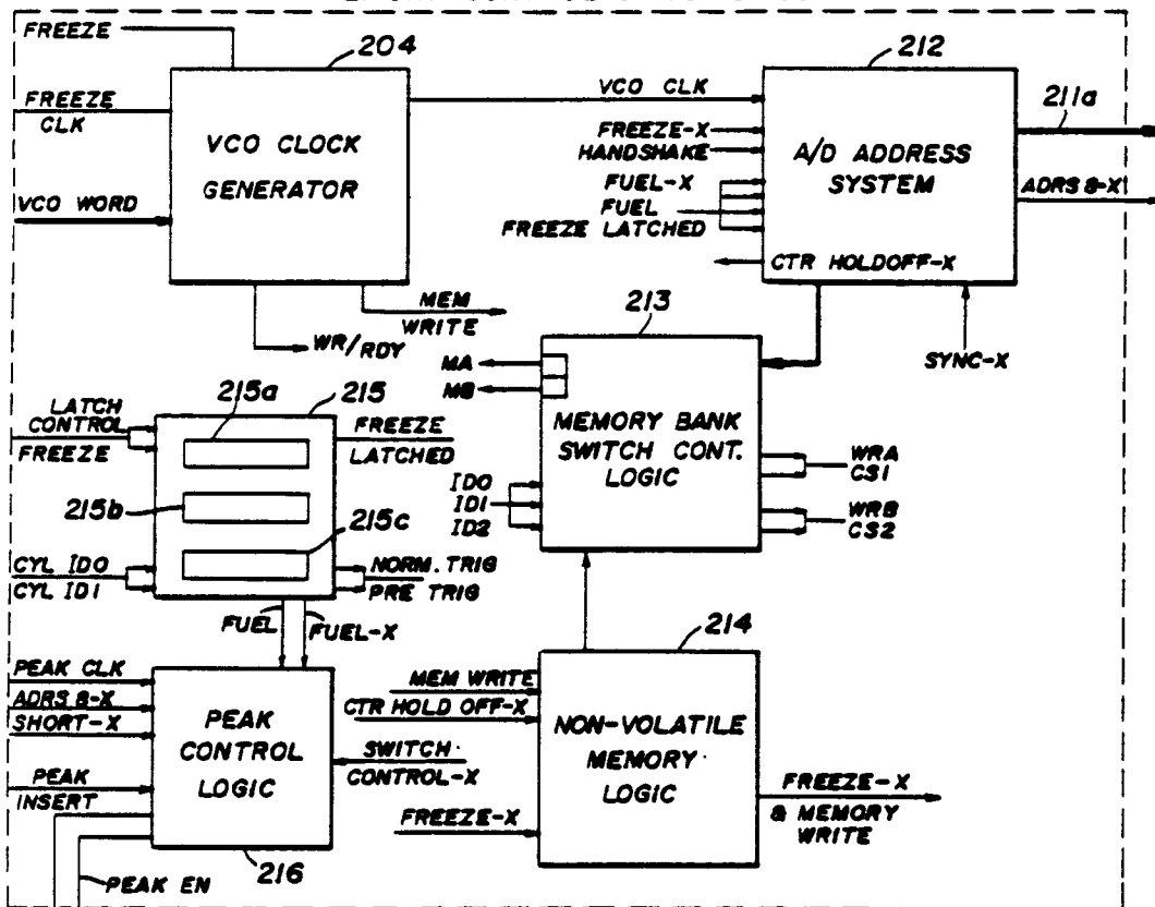
FIG. 18 MEMORY CONTROL CIRCUITS 160
