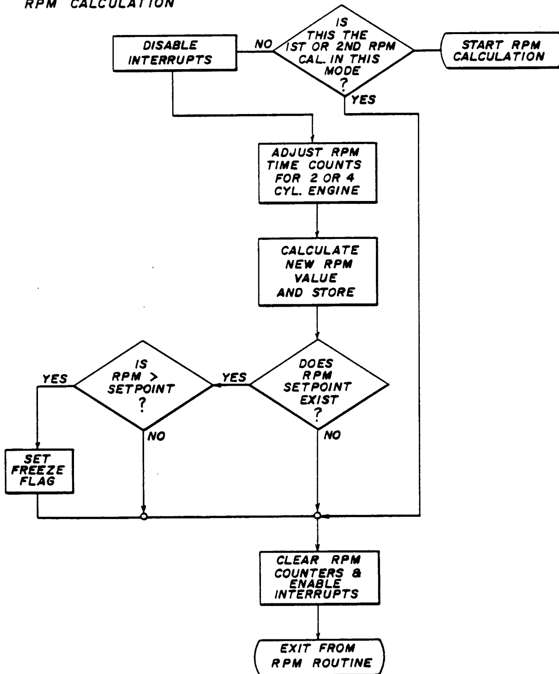
FIG.41C RPM CALCULATION
