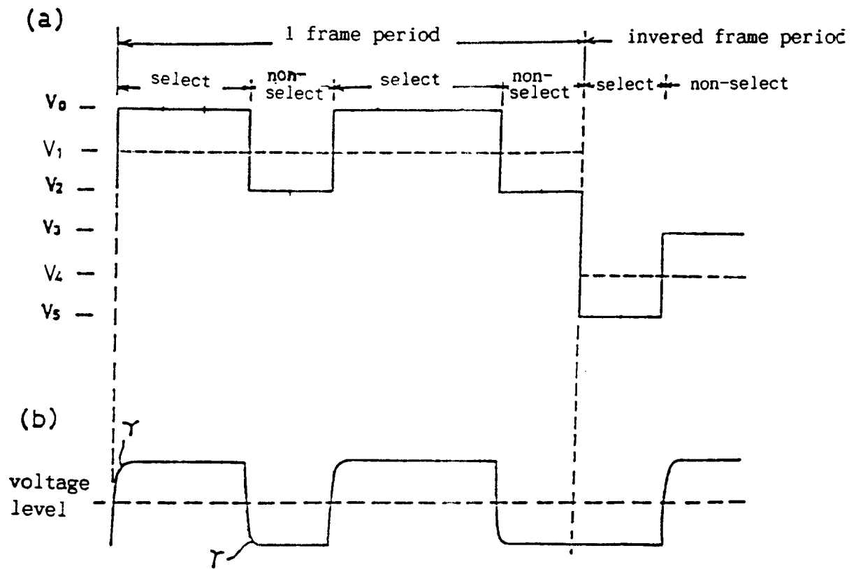
FIG. 27 (PRIOR ART)
