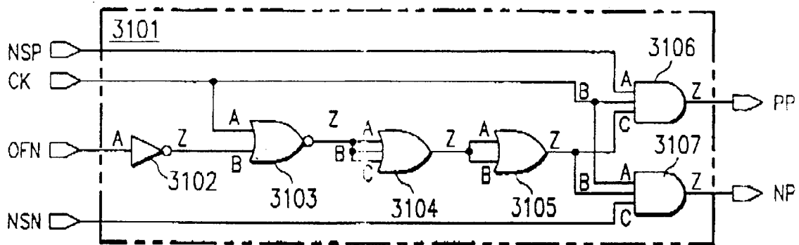
FIG. 31 PULSE GENERATOR
