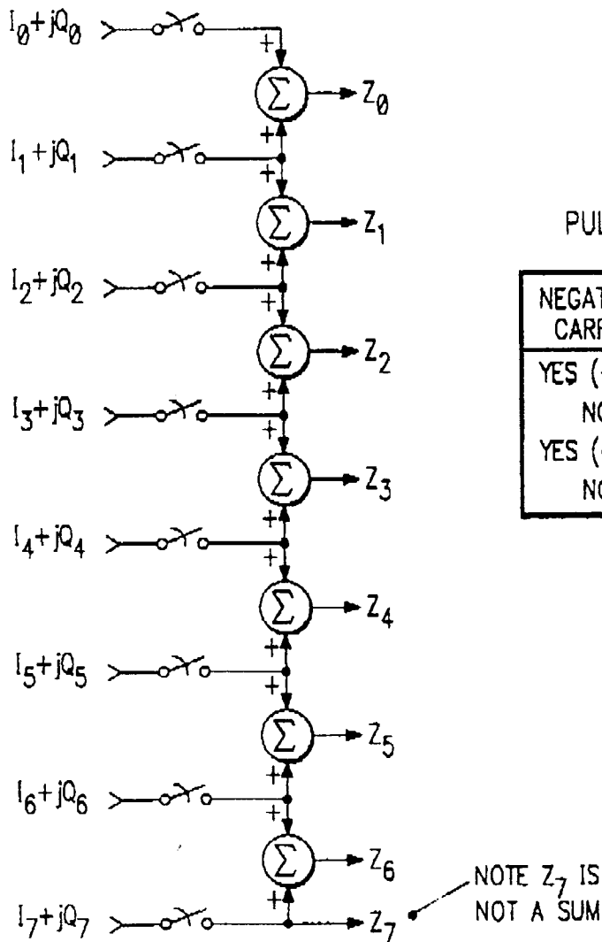
FIG. 44 ADJACENT CORRELATOR PRESUMING
