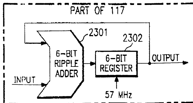
FIG. 23 (PRIOR ART)
