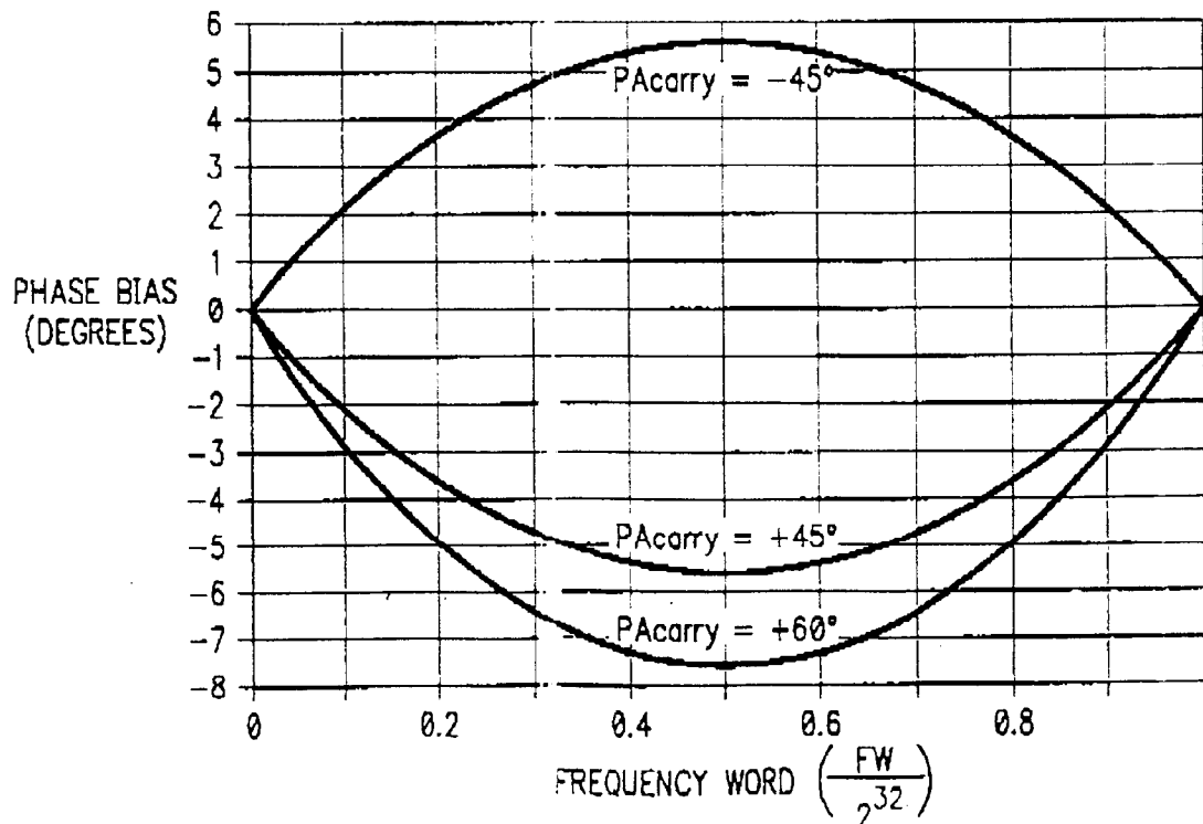
CARRY DELAY APPROXIMATION PHASE BIAS
