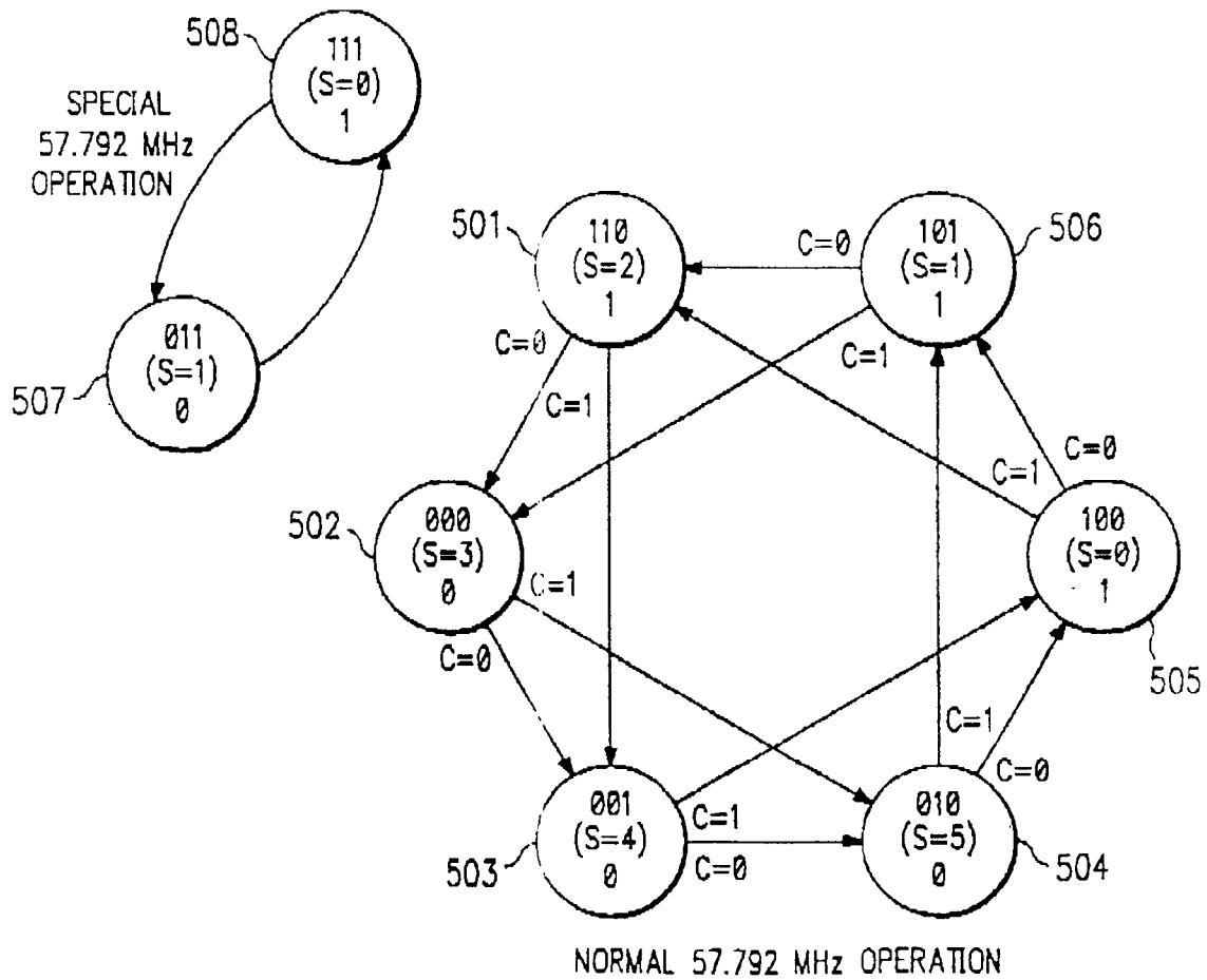
CODE CLOCK STATE DIAGRAM FOR 57.792 MHz PLAN
