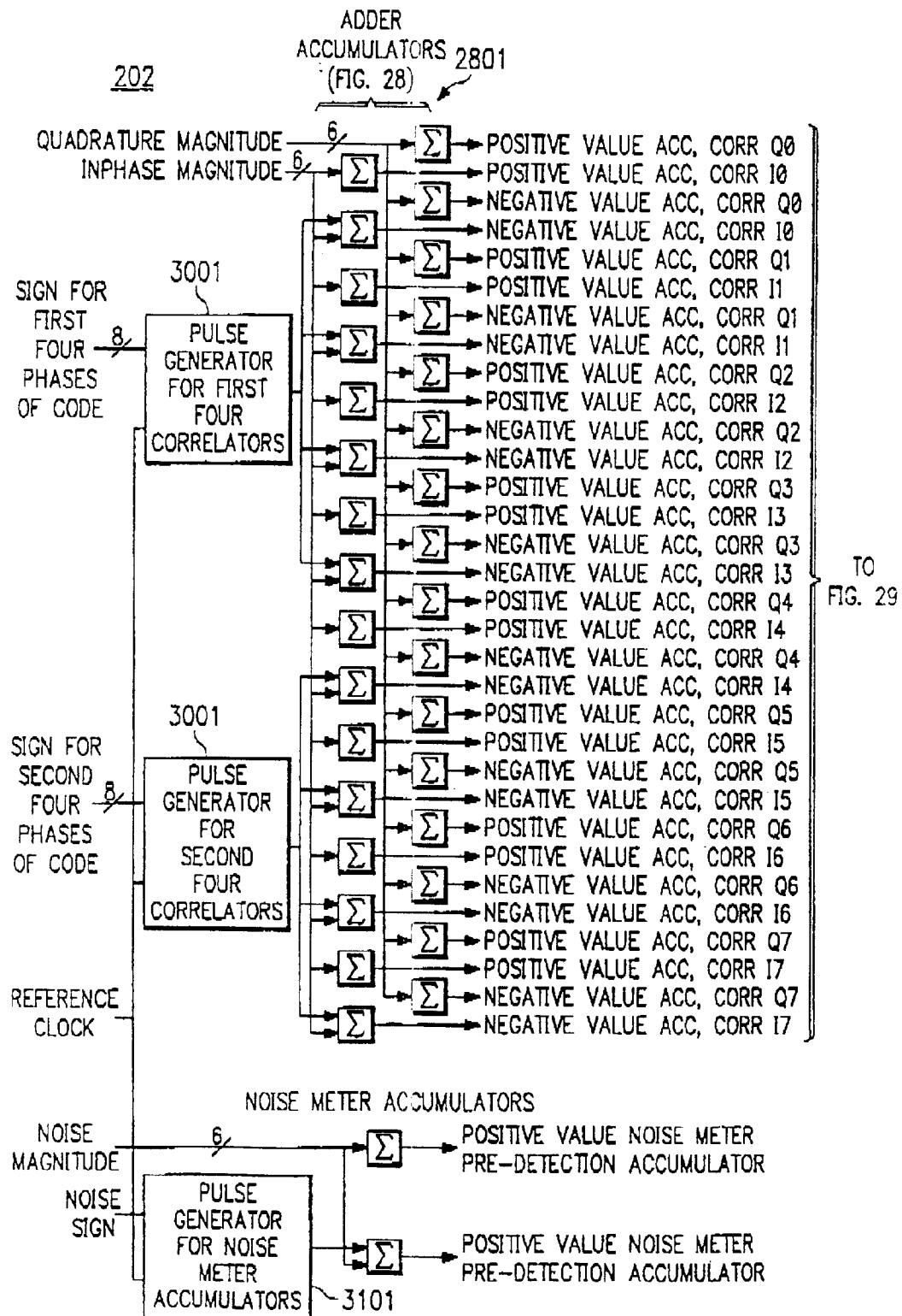
FIG. 29 INTERMEDIATE CORRELATOR MODULE BLOCK DIAGRAM
