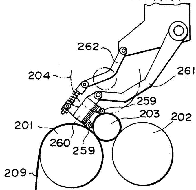
FIG. 17 PRIOR ART
