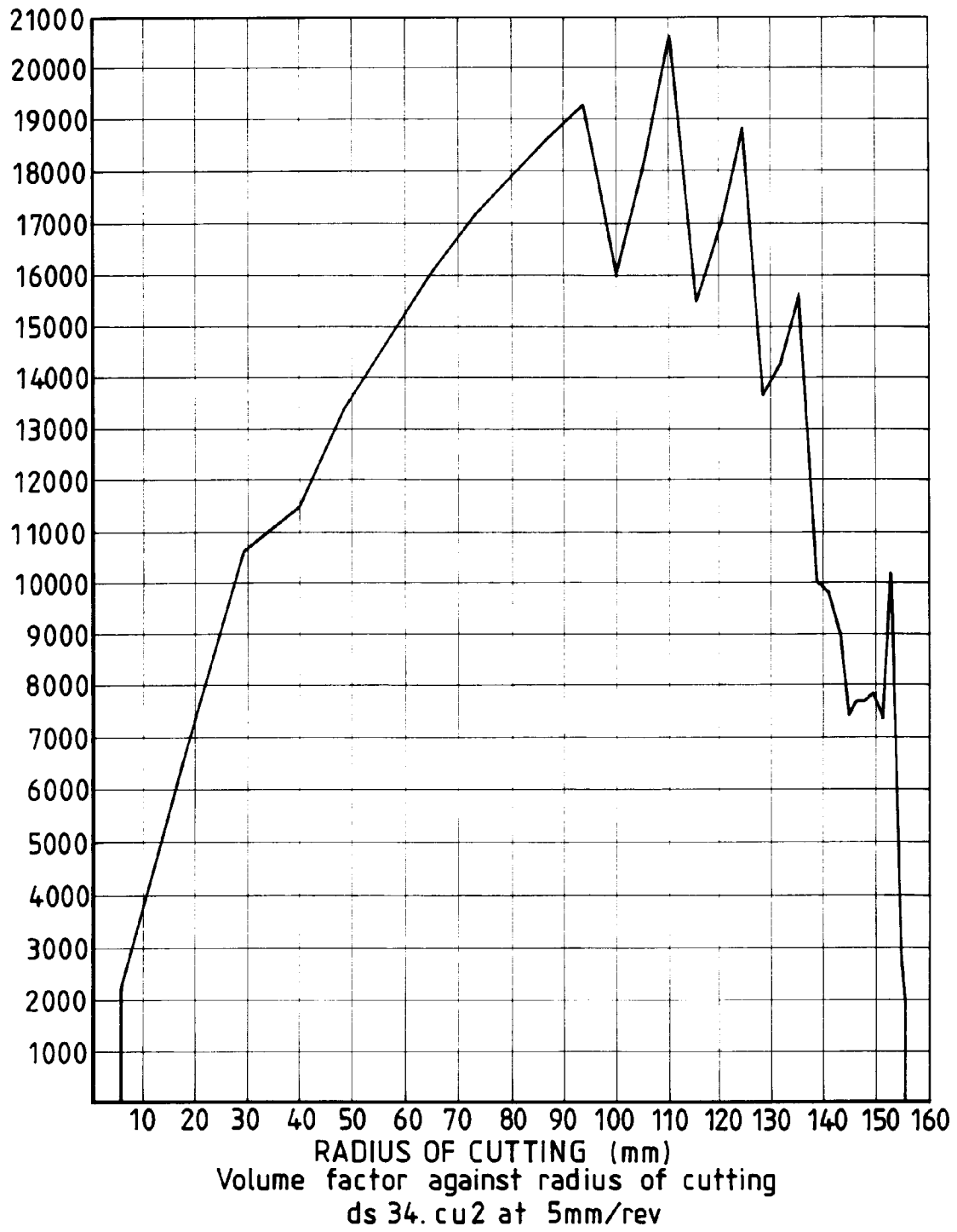
FIG 2 (Prior Art)
