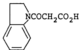
Intermediate B
