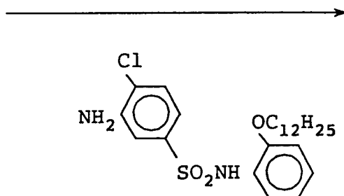
Compound E
