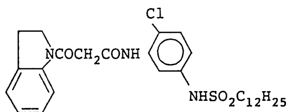
Intermediate F
