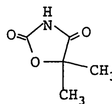
Compound D
