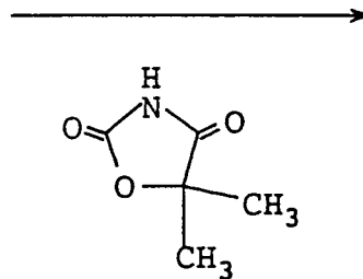
Compound D
