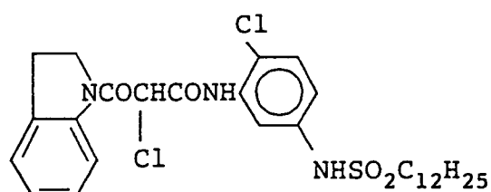
Intermediate G
