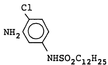
Compound F
