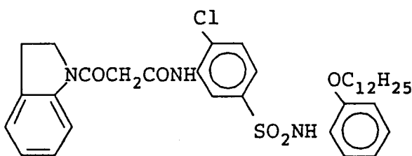
Intermediate E
