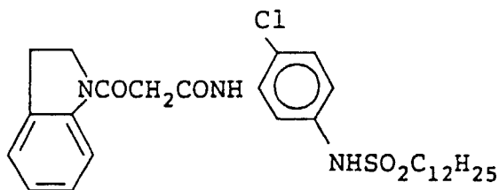
Intermediate F
