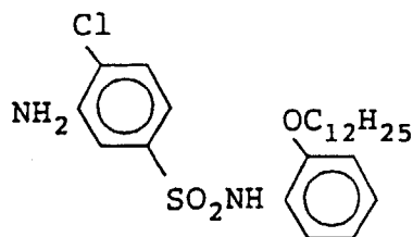
Compound E
