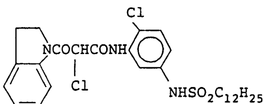
Intermediate G
