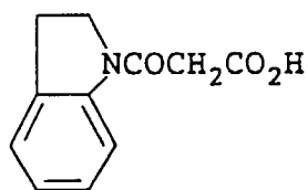
Intermediate B
