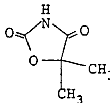
Compound D
