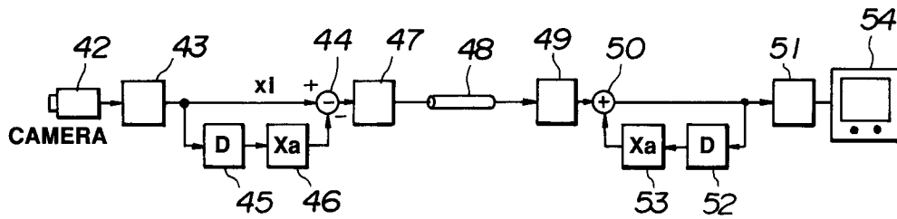
FIG.22 (RELATED ART) (a)
