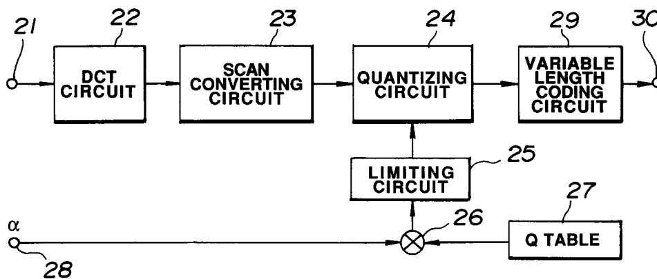
FIG.28 (RELATED ART)
