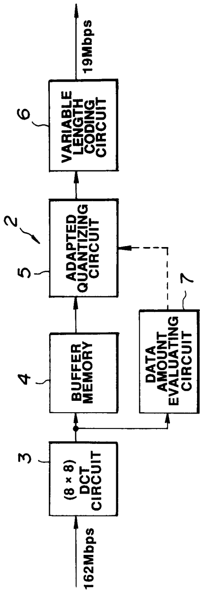
FIG.26 (RELATED ART)
