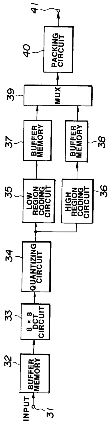
FIG.30 (RELATED ART)
