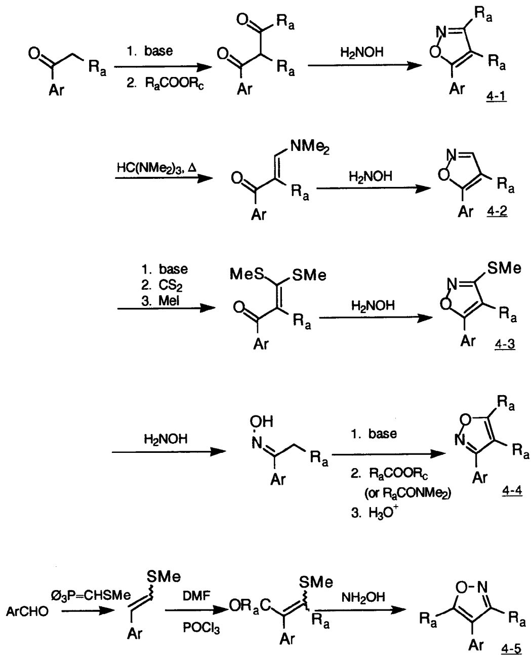
Scheme 4
