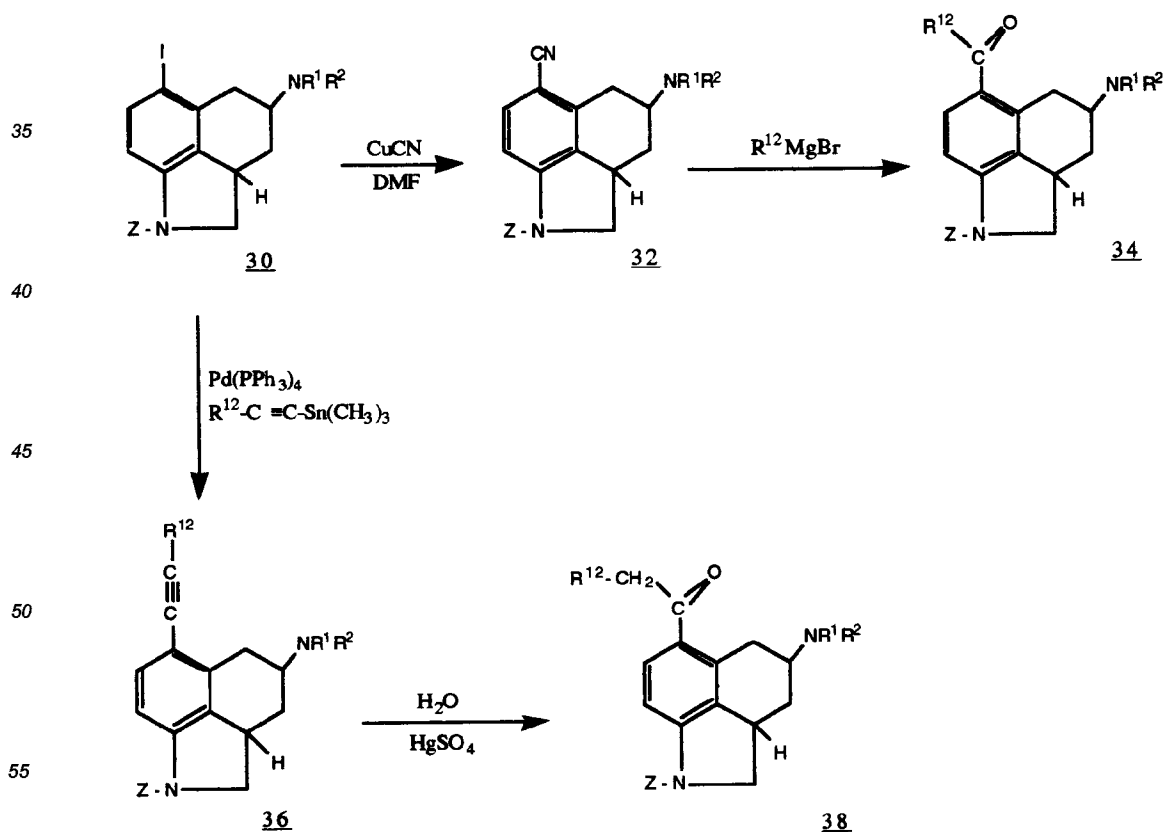
Scheme 20
