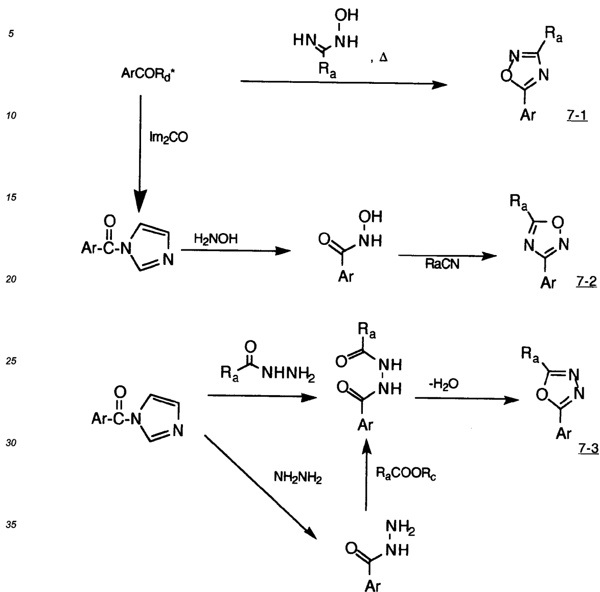
Scheme 7
