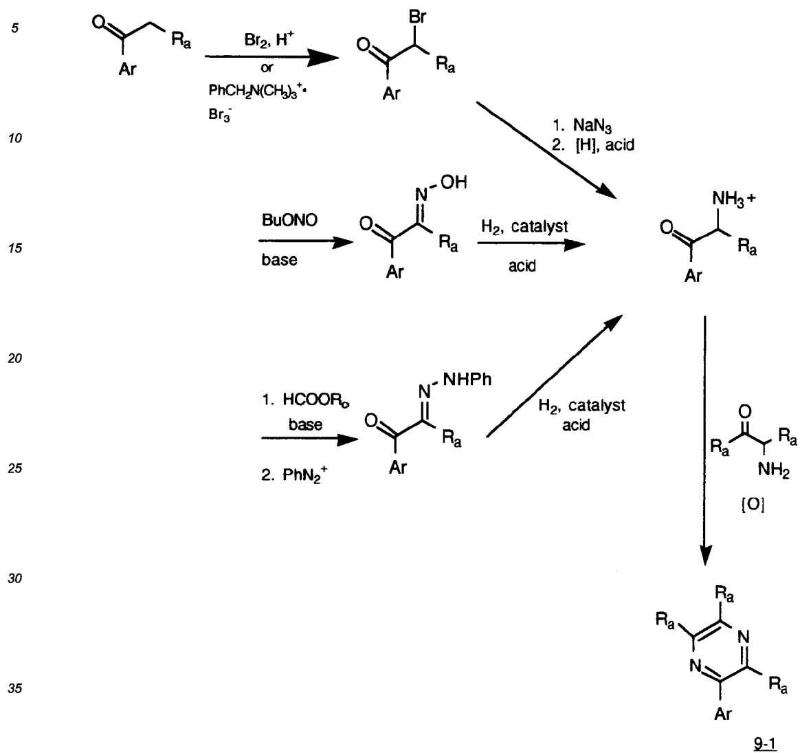
Scheme 9
