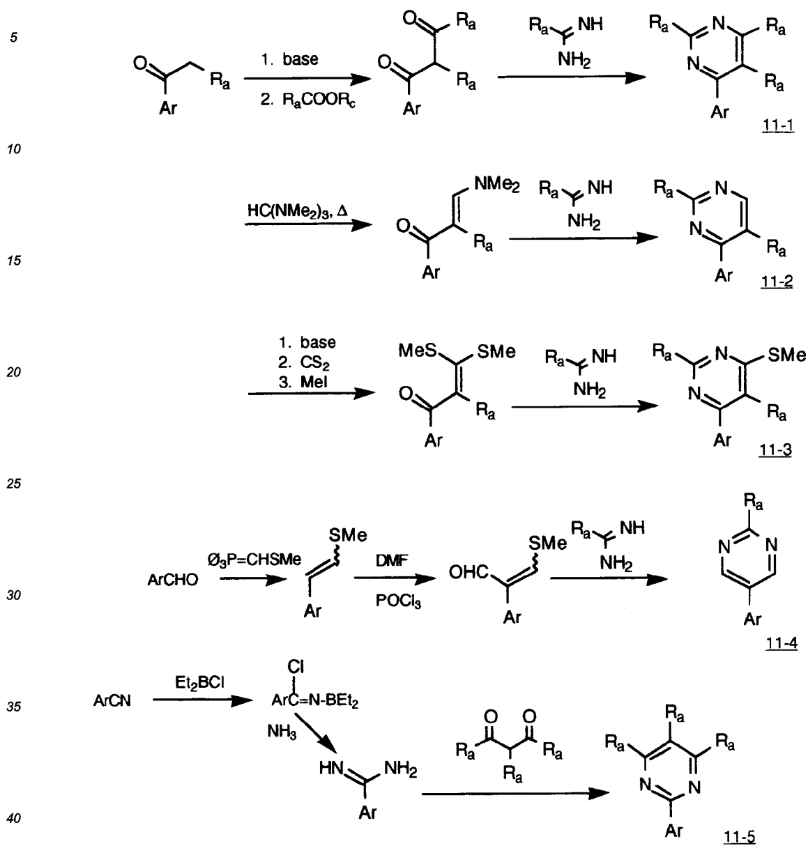
Scheme 11
