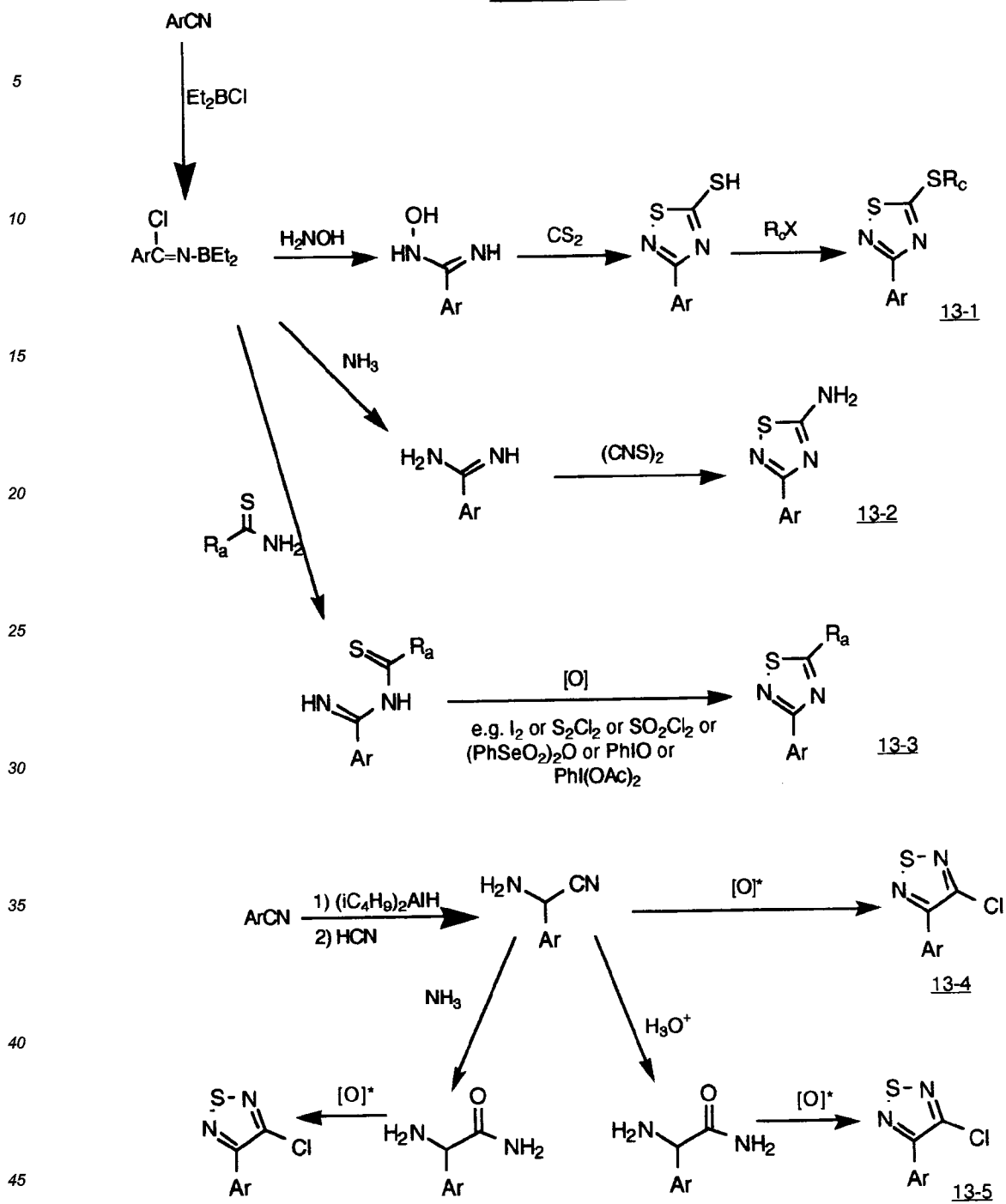
Scheme 13
