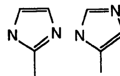
Imidazoles
