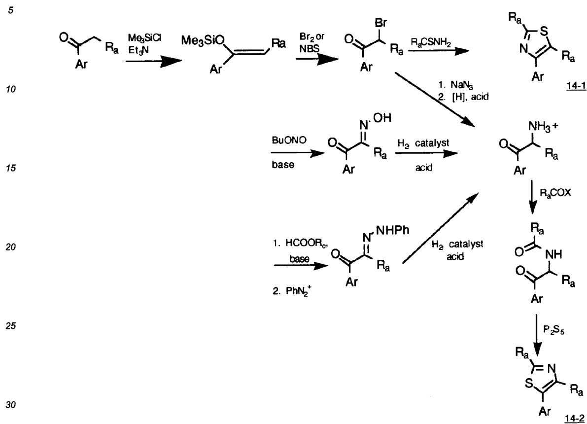
Scheme 14
