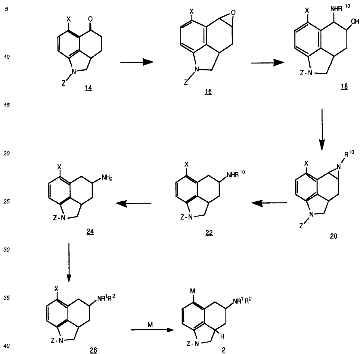
Scheme 19
