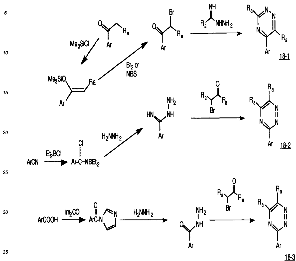
Scheme 18
