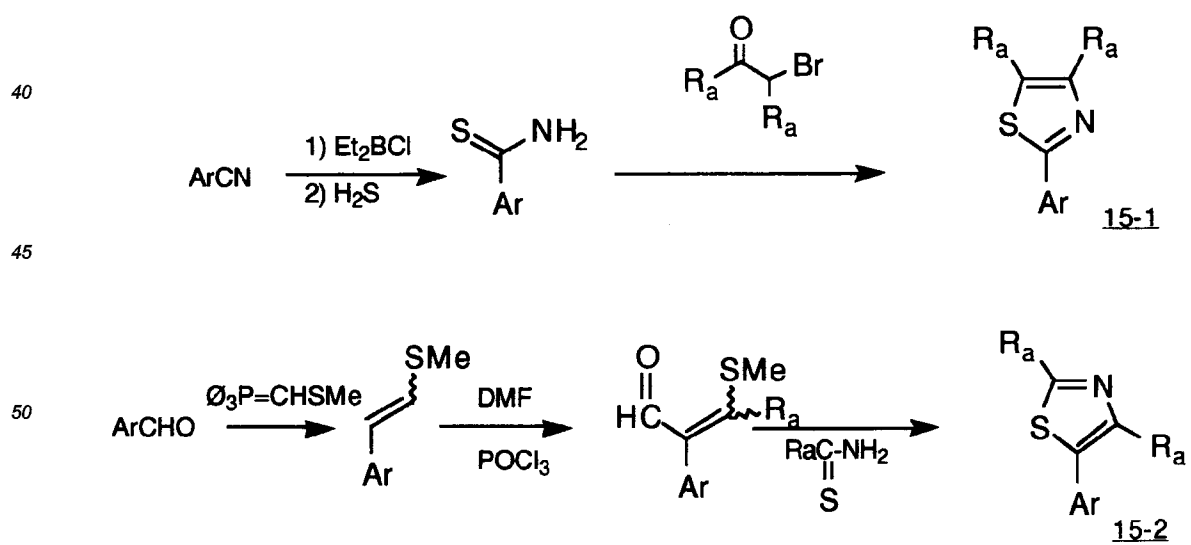
Scheme 15
