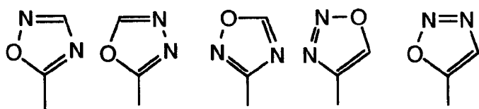
Oxadiazoles
