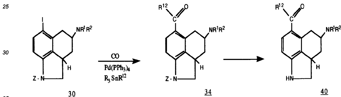
Scheme 21
