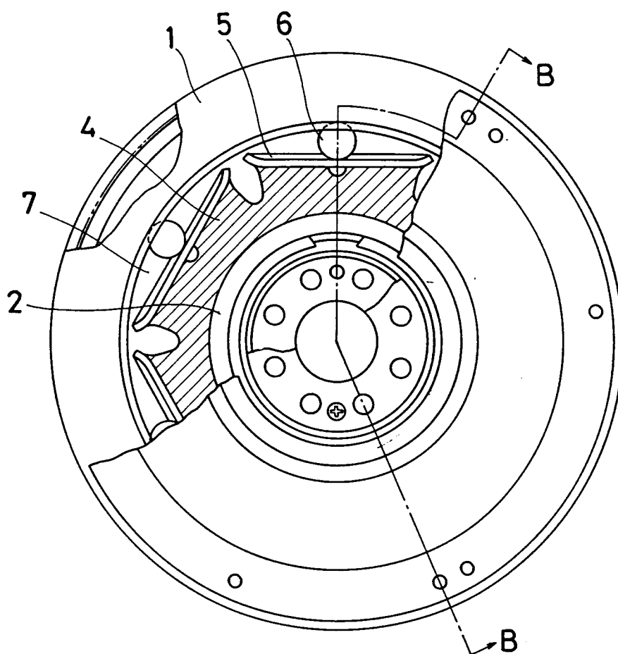
Fig. 3 (PRIOR ART)
