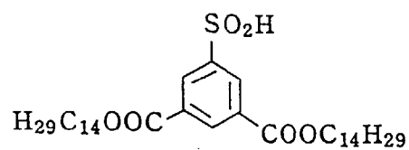
(Cpd-3) Image-dye stabilizer
