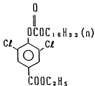
(Cpd-1) Image-dye stabilizer
