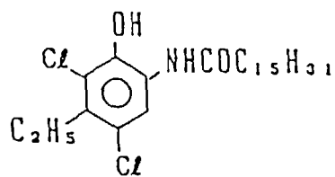
(Cpd-1) Image-dye stabilizer
