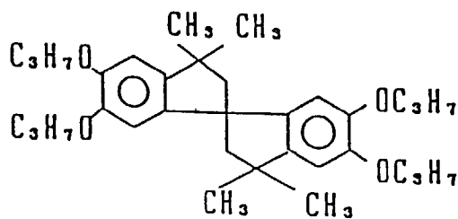
(Cpd-2) Image-dye stabilizer
