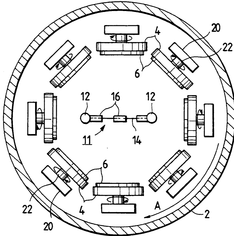
FIG. 17 PRIOR ART
