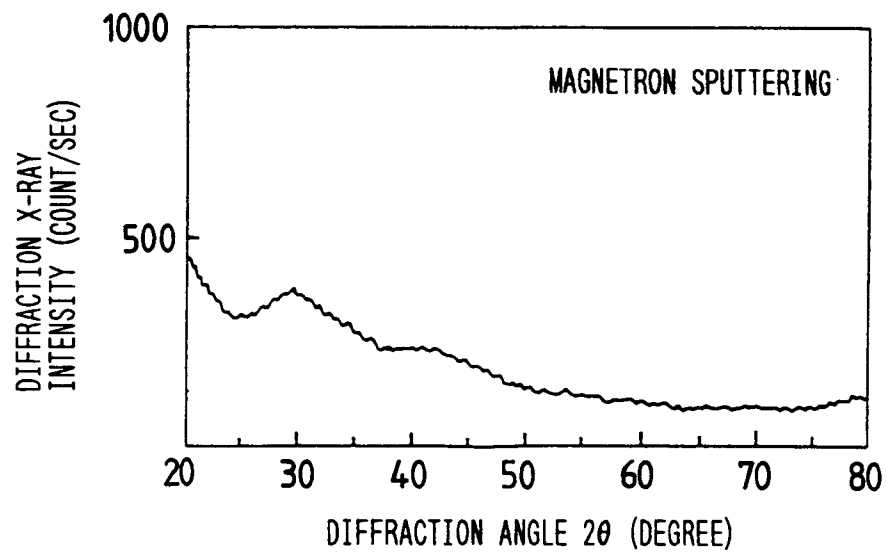
FIG. 14 PRIOR ART
