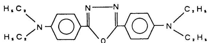
(Chemical formula 19)
