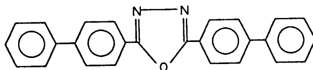
(Chemical formula 21)
