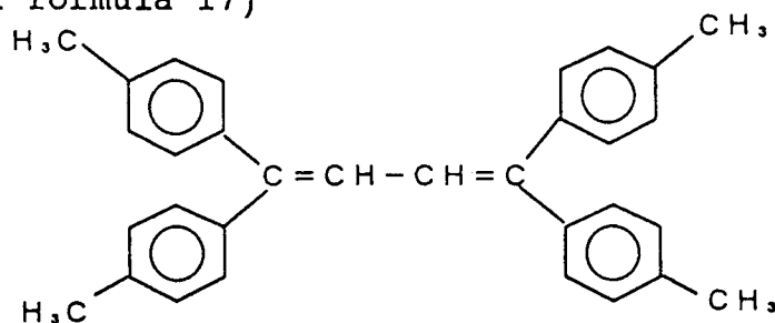
(Chemical formula 17)
