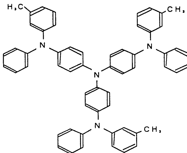
(Chemical formula 3)
