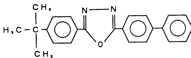
(Chemical formula 18)
