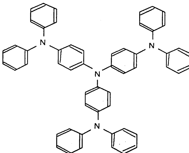
(Chemical formula 3)
