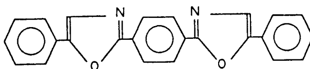
(Chemical formula 27)
