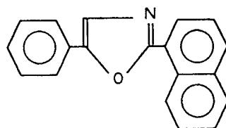
(Chemical formula 26)
