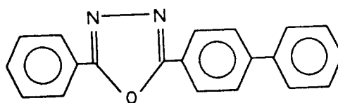
(Chemical formula 21)
