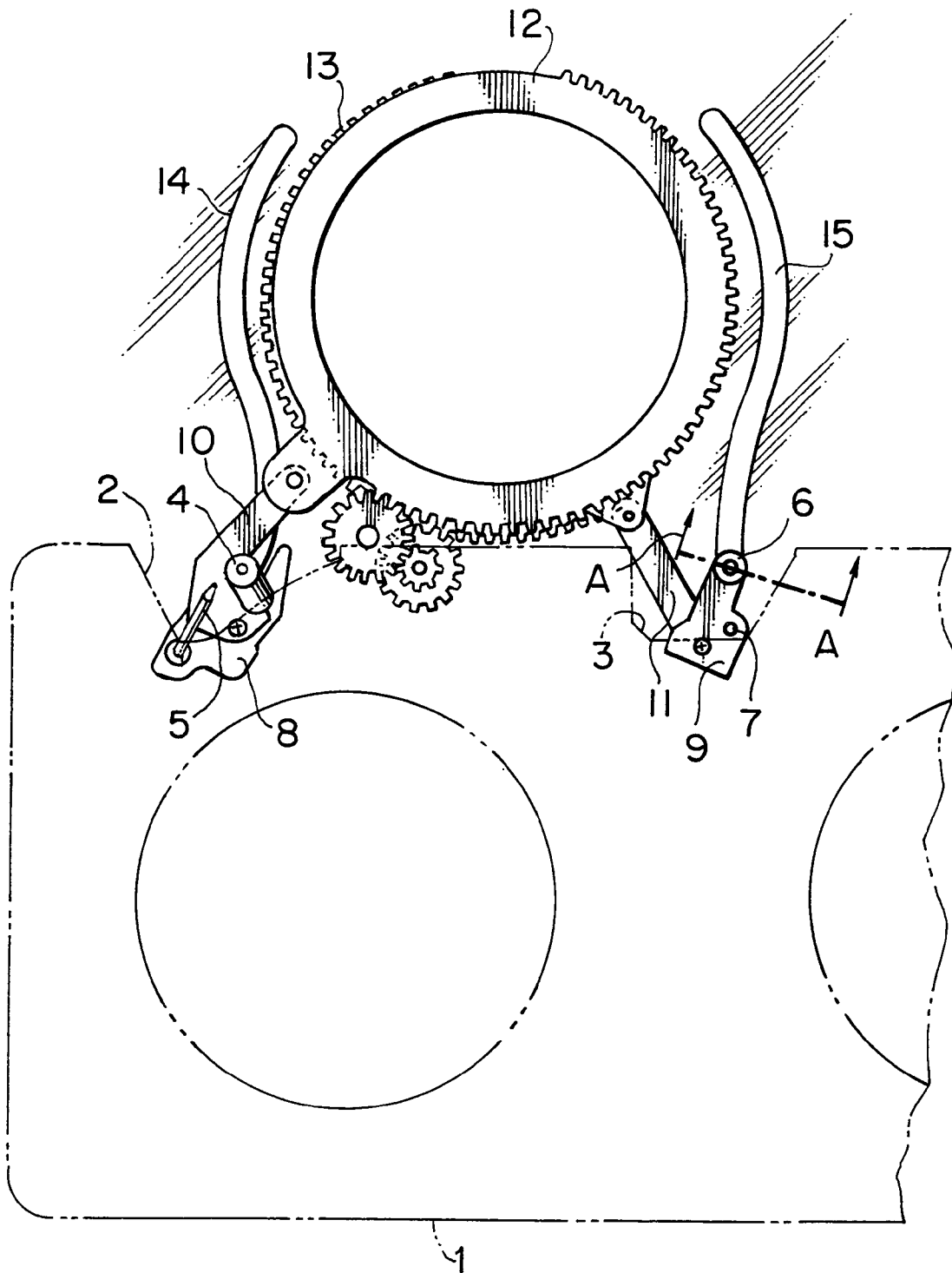
FIG. 15 PRIOR ART
