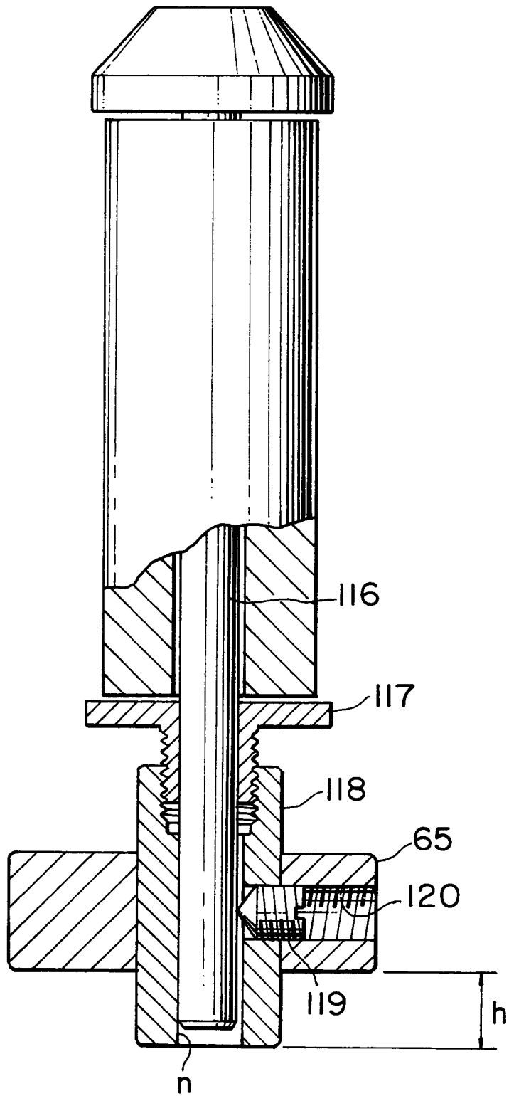
FIG. 22 PRIOR ART
