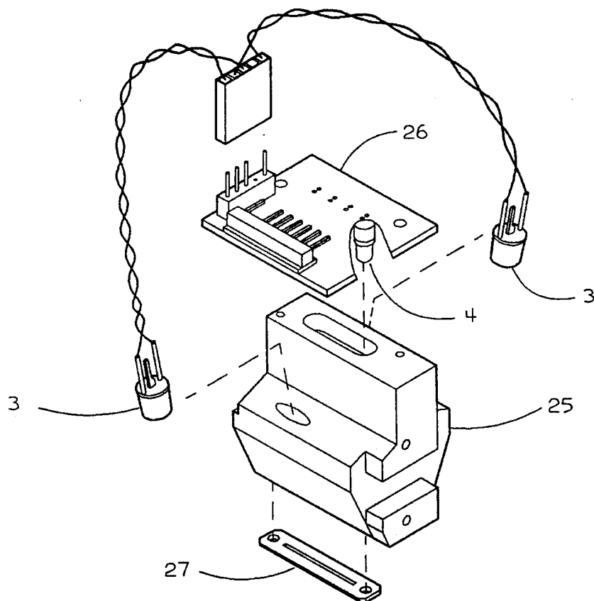
PERSPECTIVE VIEW
