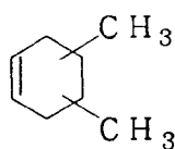
dimethylcyclohexene
