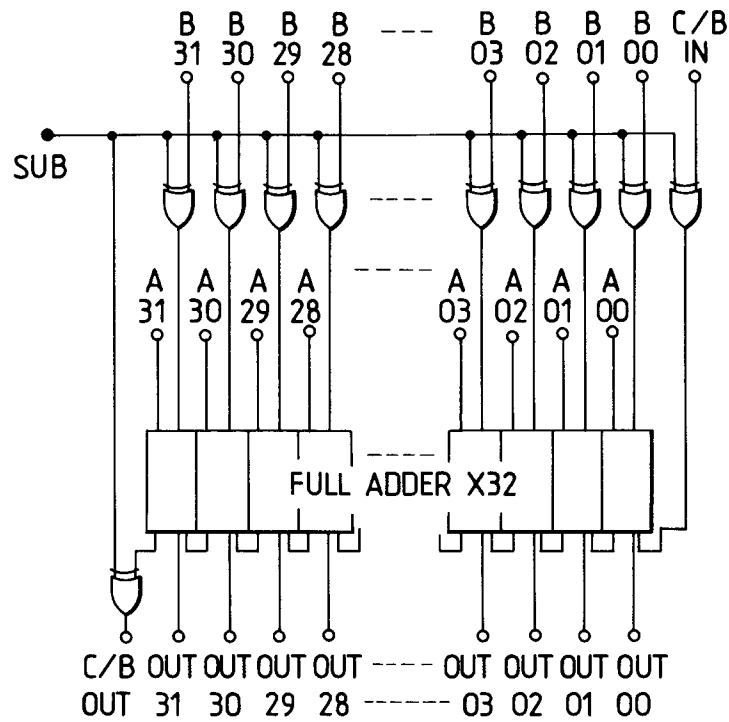
(a) ARITHMETIC LOGIC OPERATION CIRCUIT
