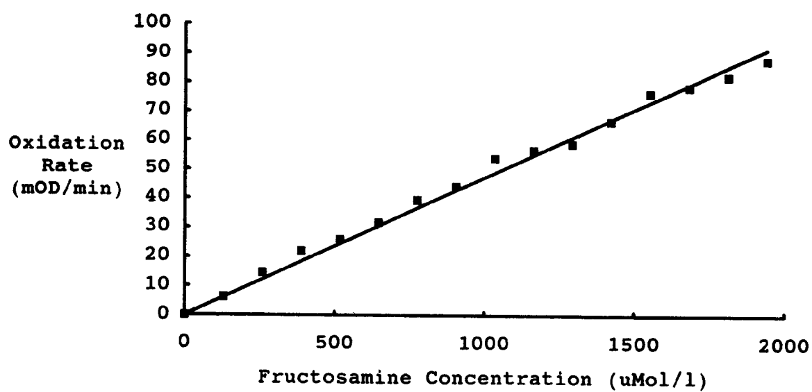
Figure 6: Fructosamine Standard Curve Kinetic Assay.
