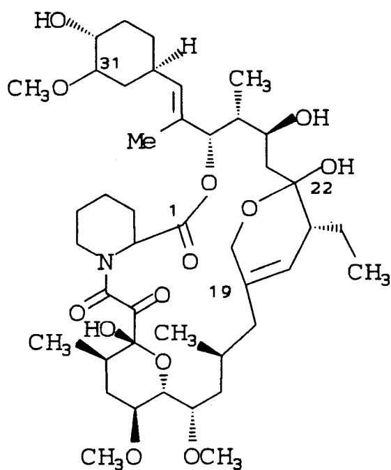
Compound II
