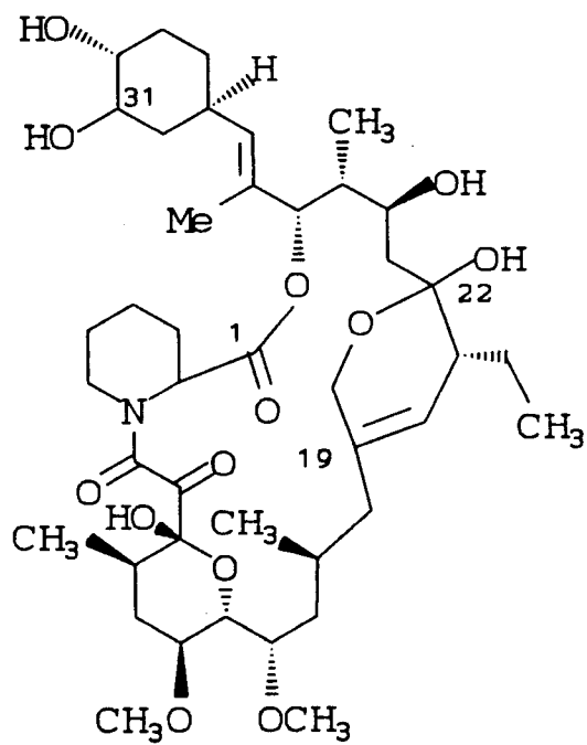
Compound I
