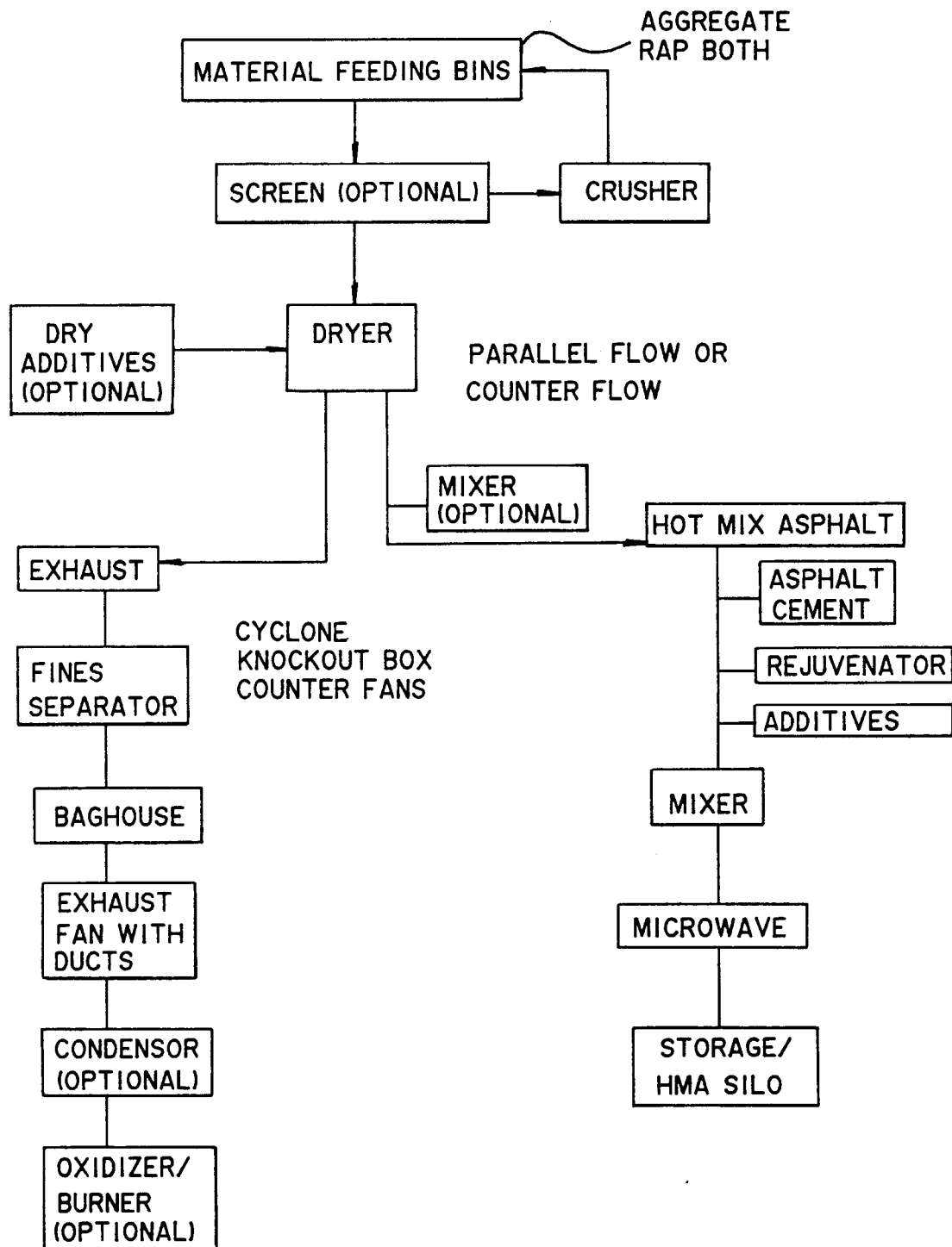
SYSTEM CONFIGURATION FOR HOT MIX ASPHALT PLANT
